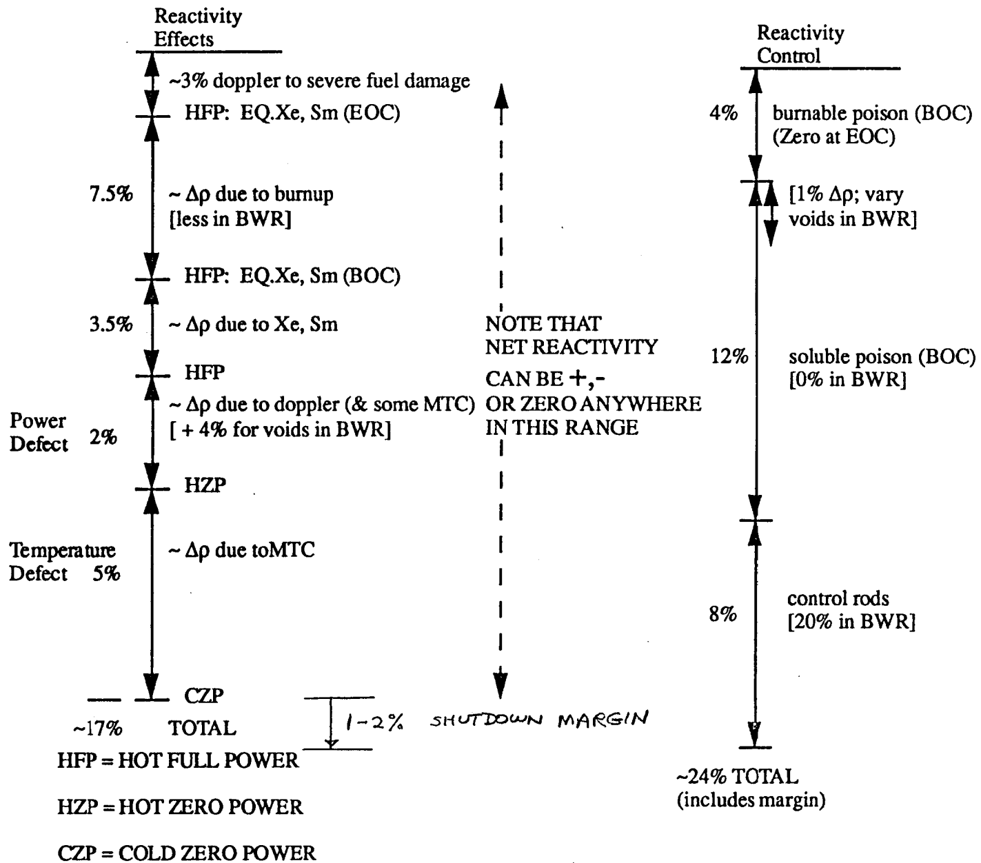
FIGURE APPROXIMATE REACTIVITY LADDER FOR LWR
