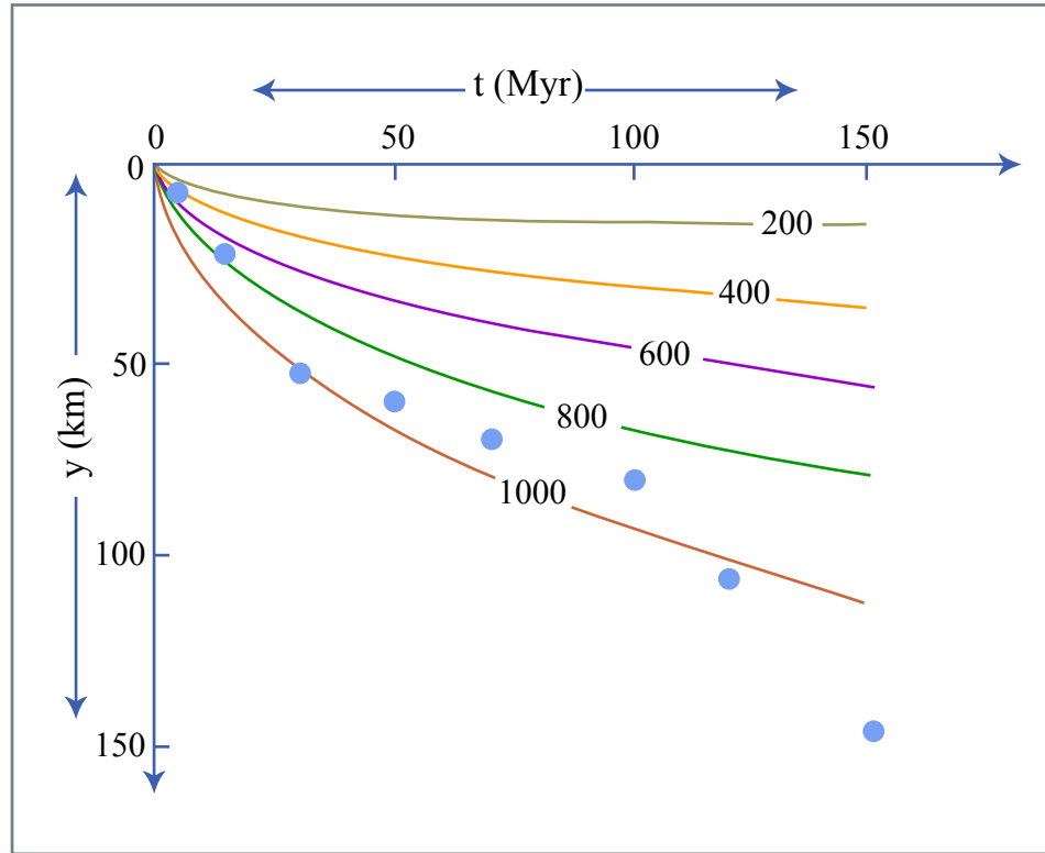
Figure 5.9: Oceanic geotherms.
