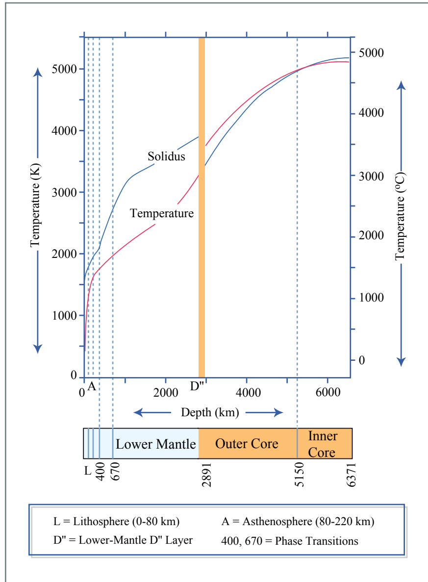
Figure 5.3: Geotherms in the Earth.
