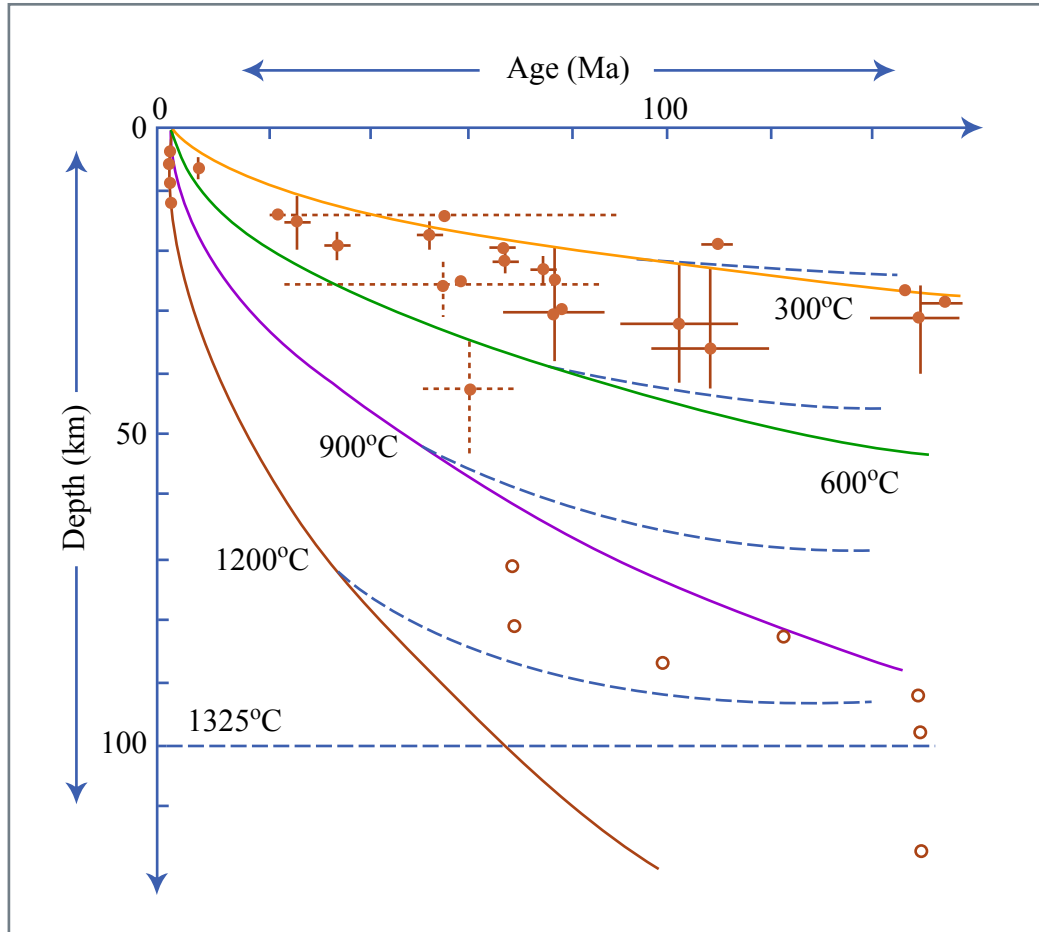
Figure 5.10: Elastic thickness.
