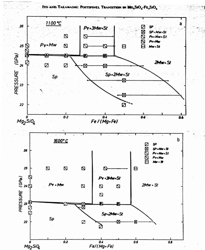
Figure 5.22: Phase diagrams of mineral transformations in the mantle.
