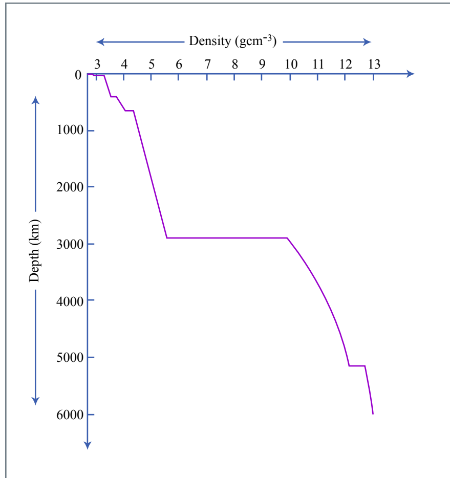
Figure 5.21: The density of the Earth according to model ak135 .
