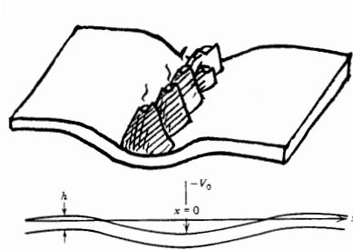
Figure 5.16: Deflection of an elastic plate under a line load.
