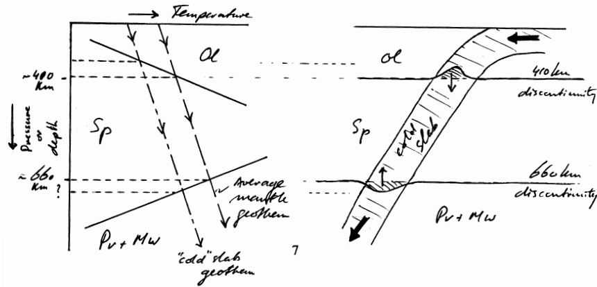
Figure 5.23: Effects of phase transformations on downgoing slabs.
