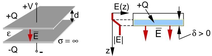
Figure R13.2. Electric charge within skin depth \delta in capacitor plates
