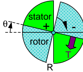
Figure R13-5. Rotary electrostatic motor
