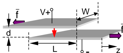
Figure R13-3. Capacitor plates separated laterally
