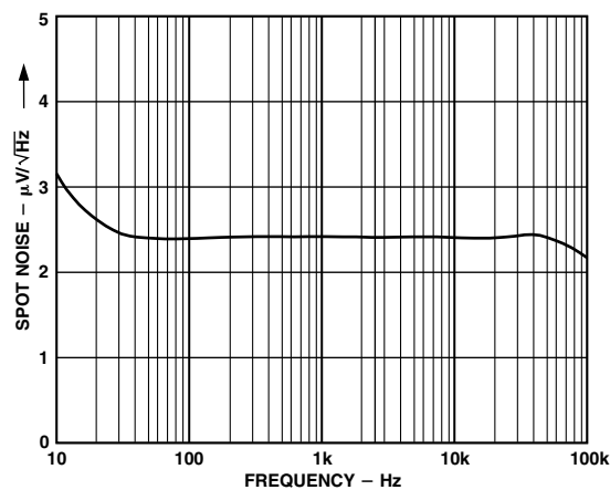
Figure 10. Spot Noise vs. Frequency
