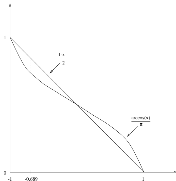
Figure 7: Calculating \alpha .
