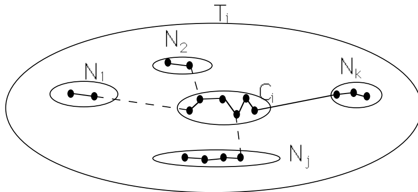
Figure 4: d_H(v) \geq 2 for v \in Even
