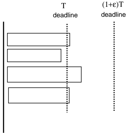
Figure 9: Scheduling “small” jobs.
