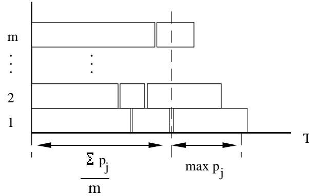
Figure 8: List scheduling.
