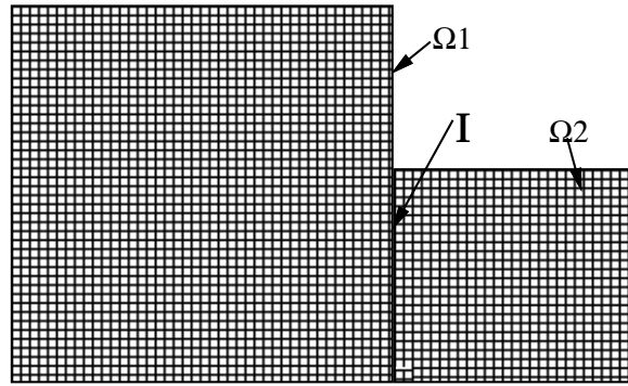
Problem Domain
