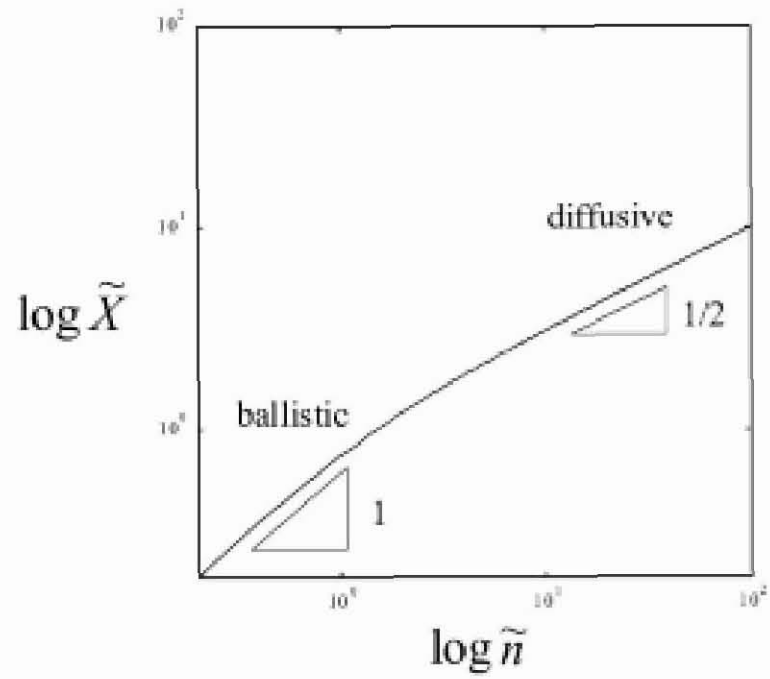
Figure 1: Ballistic-diffusive transition.
