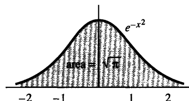
Fig. 14.9 Bell-shaped curve.
