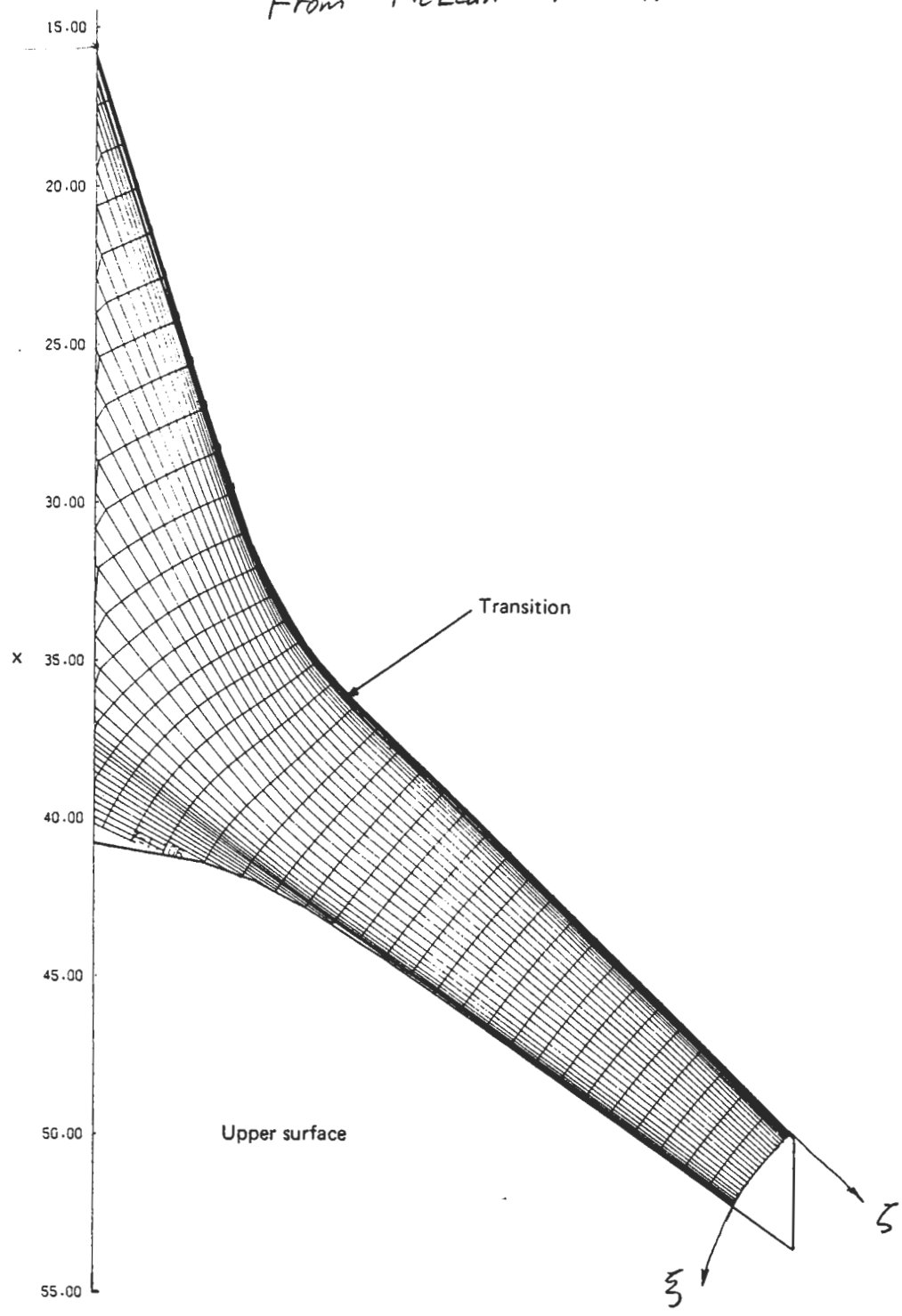
Figure 23a.—Boundary Layer Computational Grid
