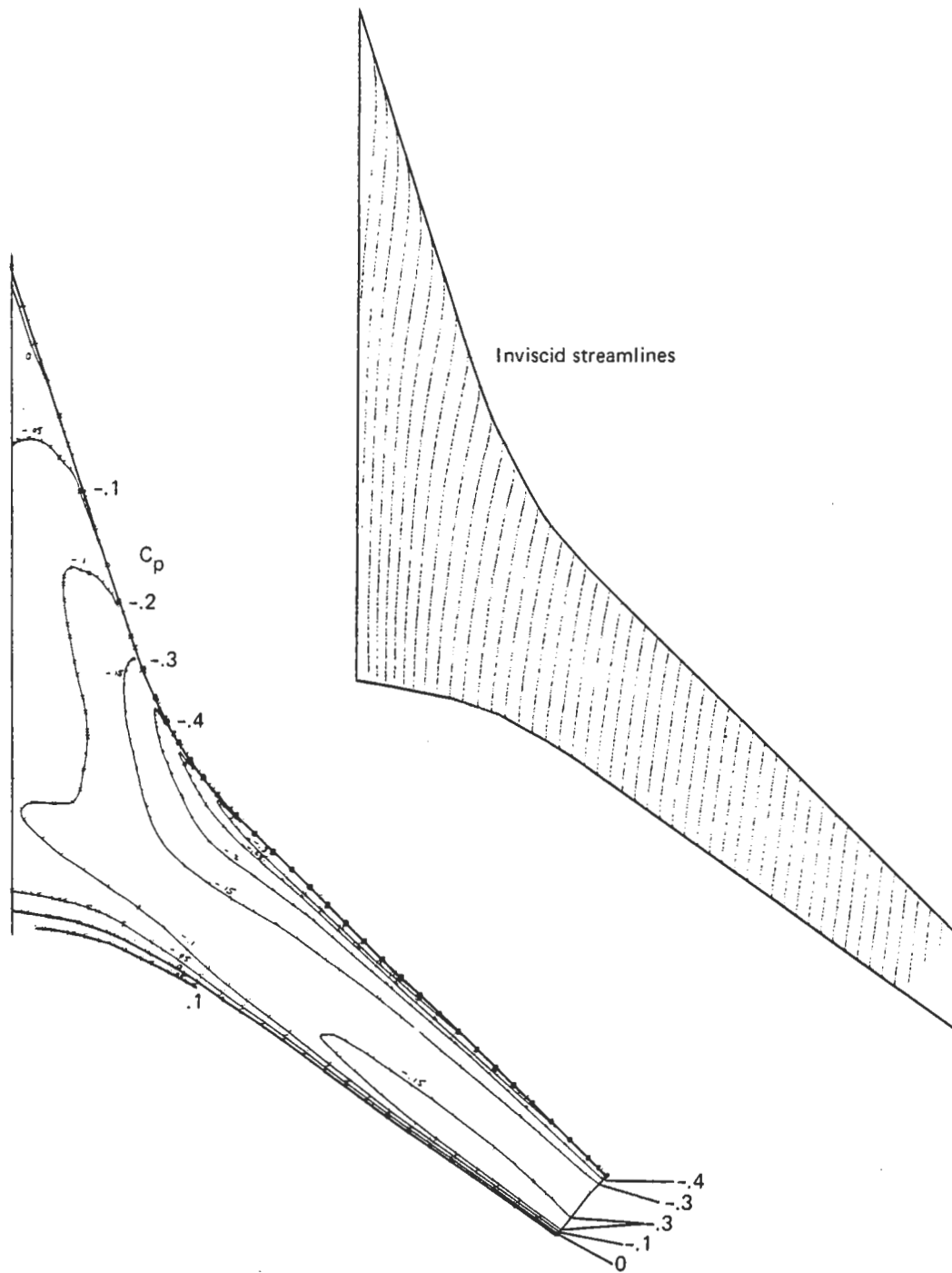
Figure 30a.—Outer Inviscid Flow Solution for Upper Surface (With Suction)
