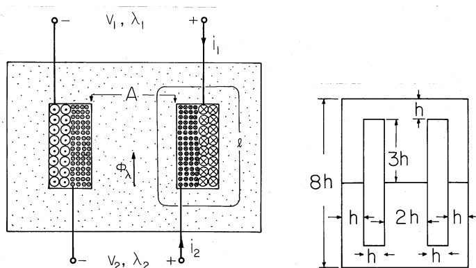
Fig. 9.7.7 In a typical transformer, coupling is optimized by wrapping the primary and secondary on the same core. The inset shows how full use is made of the magnetizable material in the core manufacture.
