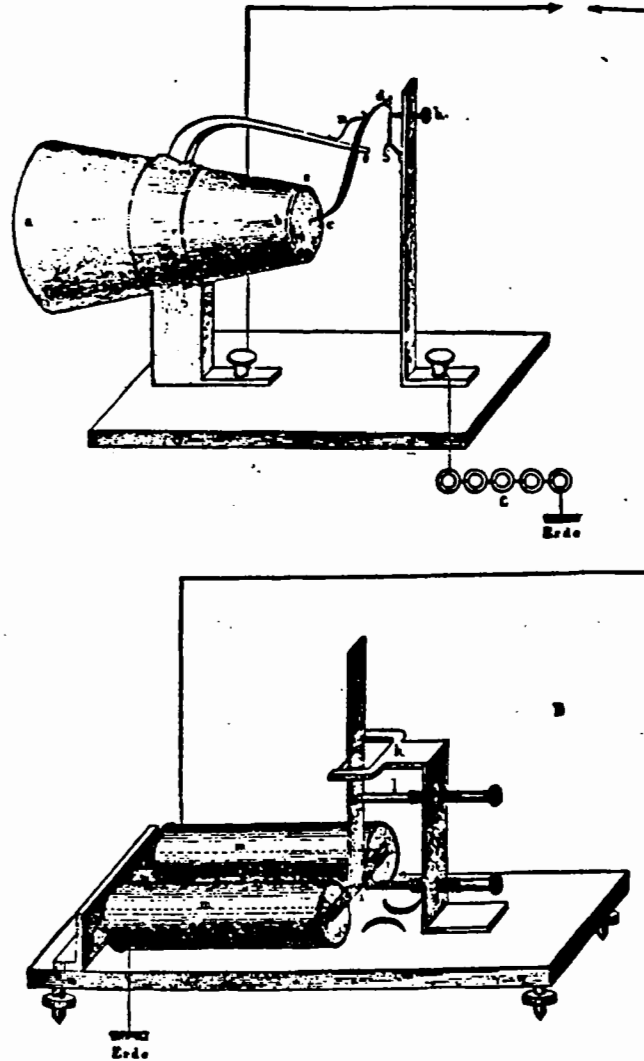
Figure 5. Philip Reis's construction.
