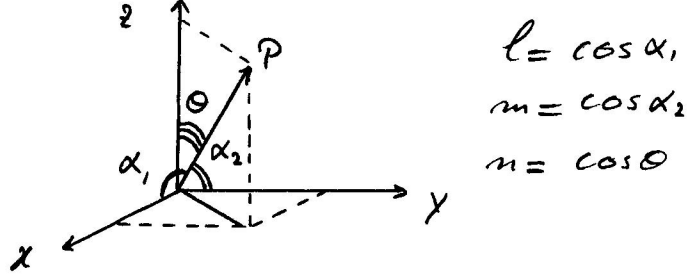
Figure 2.7: Definition of direction cosines.
