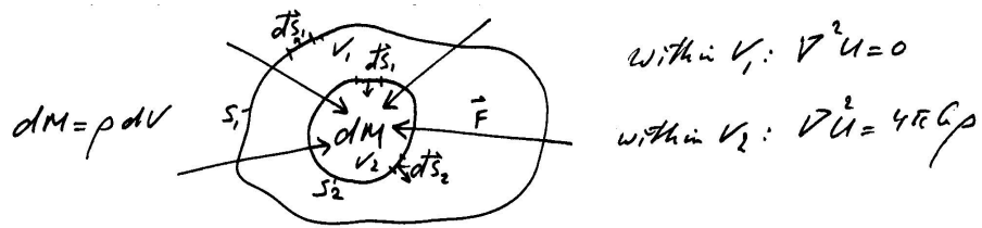
Figure 2.11: Applicability of Poisson's and Laplace's equations.
