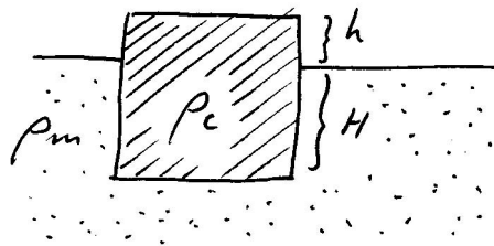
Figure 2.19: Airy isostasy.
