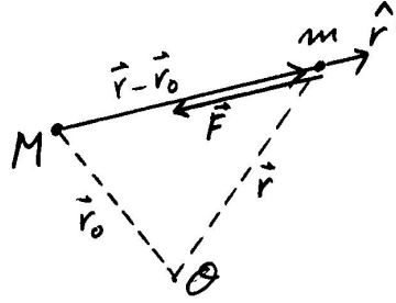
Figure 2.1: Vector diagram showing the geometry of the gravitational attraction.
