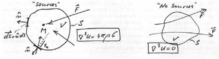
Figure 2.10: Poisson's and Laplace's equations.
