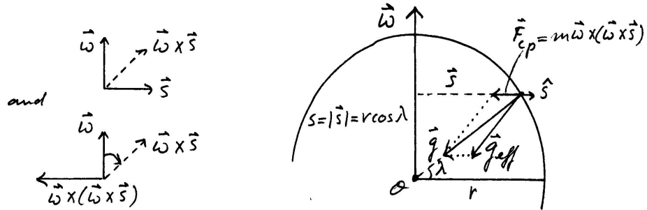
Figure 2.8: The gravitational attraction produces the centripetal force due to the rotation of the Earth.
