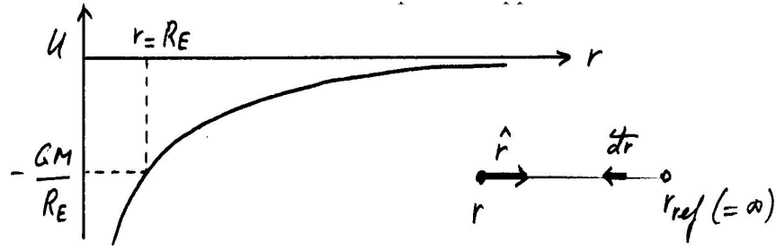
Figure 2.3: By definition, the potential is zero at infinity and decreases towards the mass.
