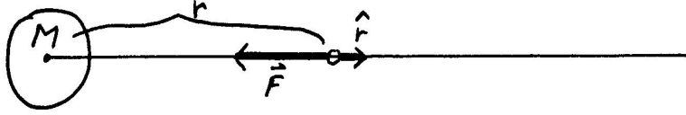
Figure 2.2: Simplified coordinate system.
