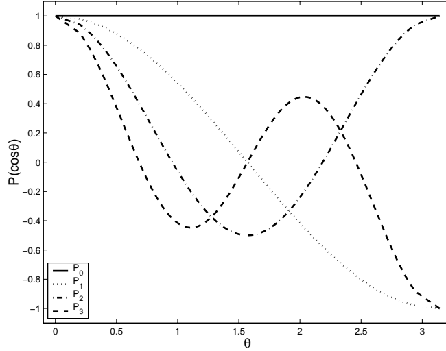
Figure 2.13: Legendre polynomials.
