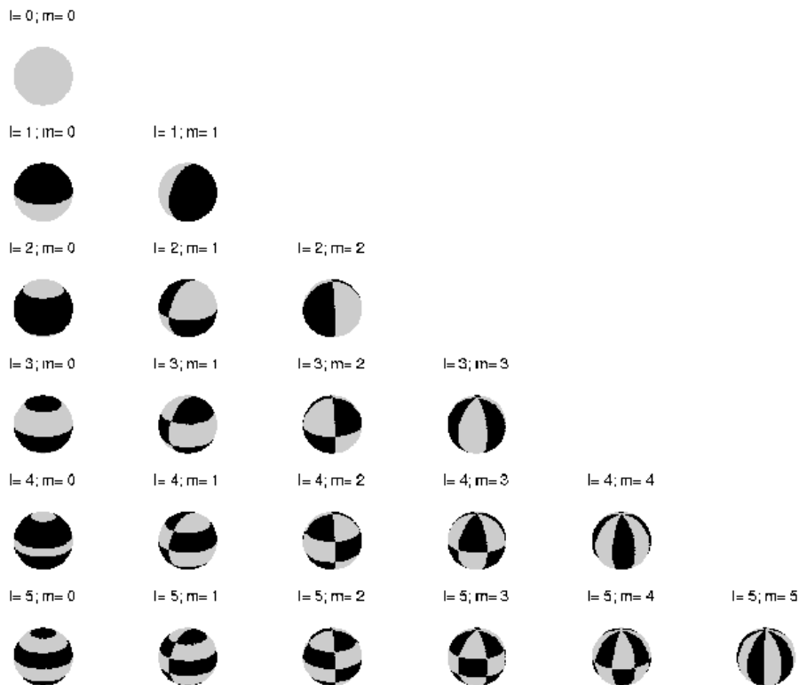
Figure 2.14: Some spherical harmonics.
