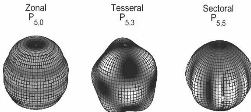
Figure 2.15: Zonal, tesseral and sectoral spherical harmonics.
