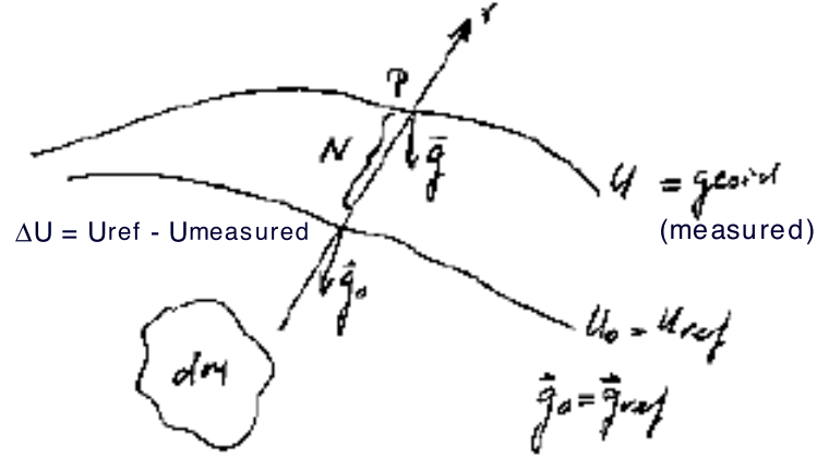
Figure 2.17: Derivation. Note that in this figure, the sign convention for the gravity is reversed; we have used and are using that the gravity is the negative gradient of the potential.
