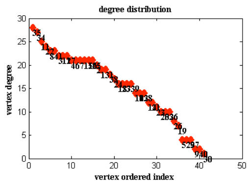
degree distribution for Roofnet (symmetrical)
