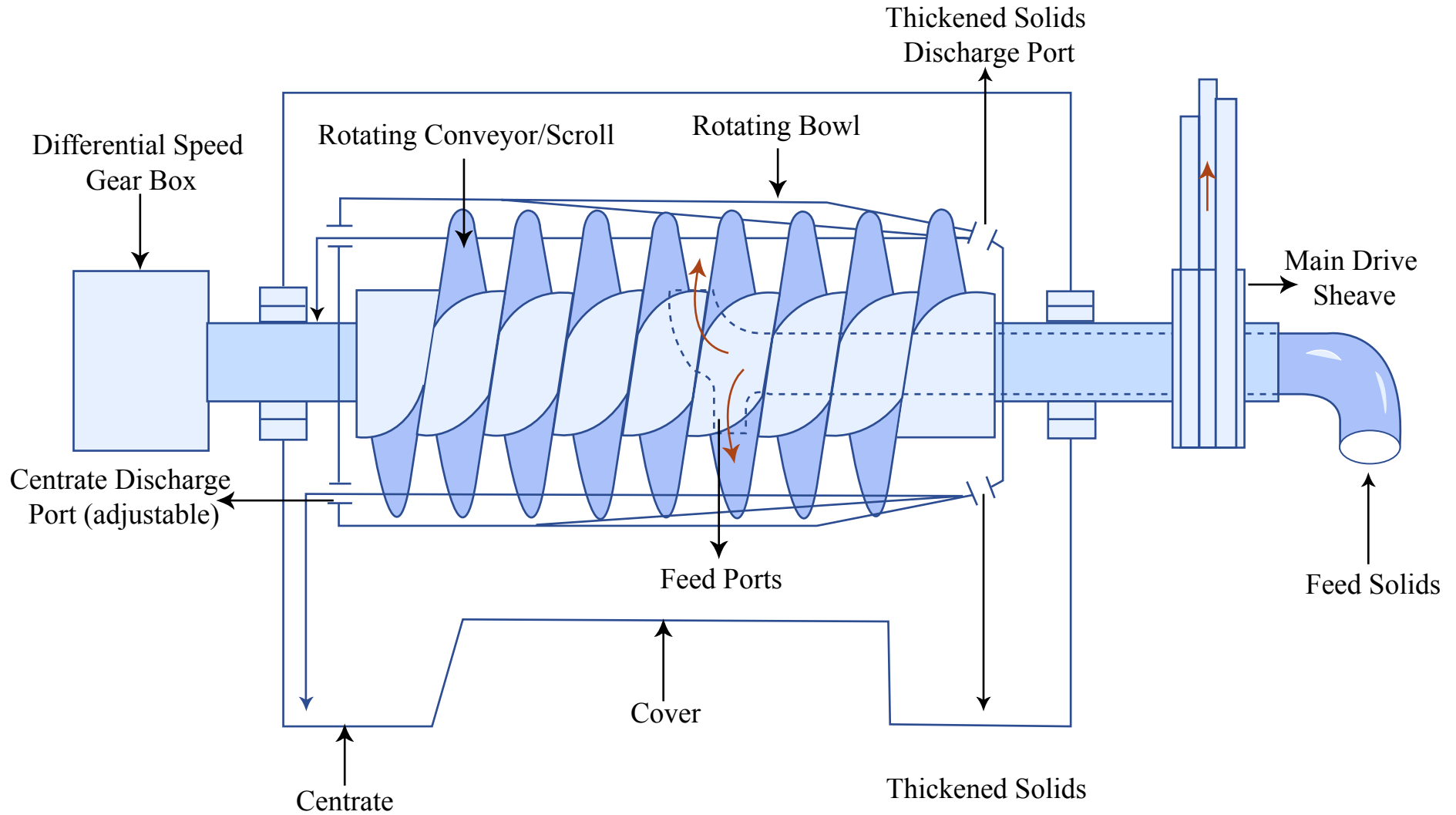
Figure by MIT OCW. Adapted from: G. Tchobanoglous, F. L. Burton, and H. D. Stensel. Wastewater Engineering: Treatment and Reuse . 4th ed. Metcalf & Eddy Inc., New York, NY: McGraw-Hill, 2003, p. 1469.
