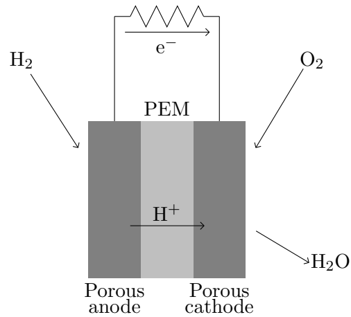
Figure 2: PEM fuel cell
