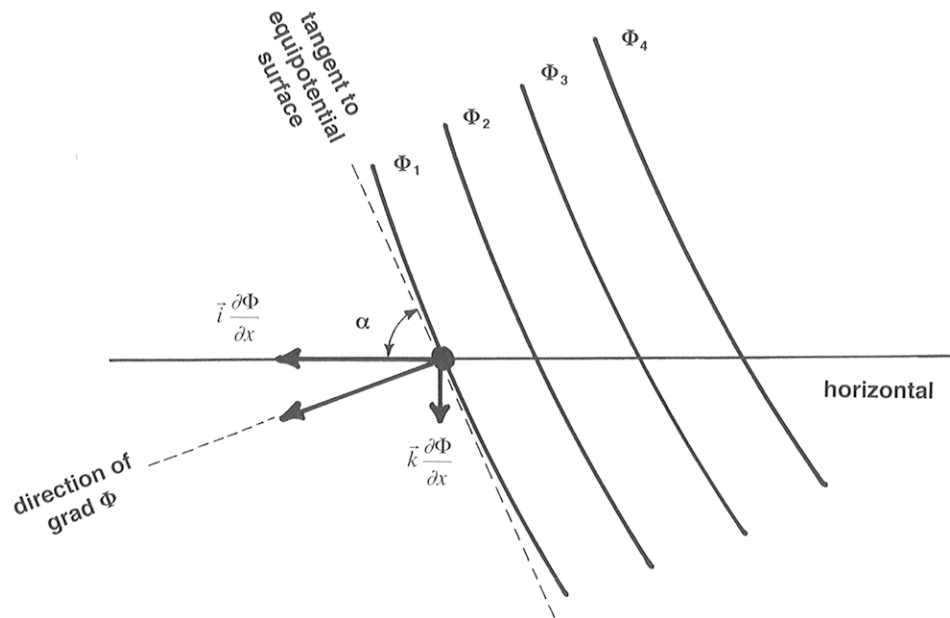
Figure 7-33. Flow of water in a glacier in response to the gradient of a potential.
