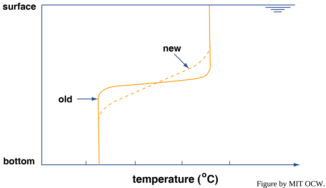
Figure 6-9. Thickening of the thermocline by molecular diffusion.
