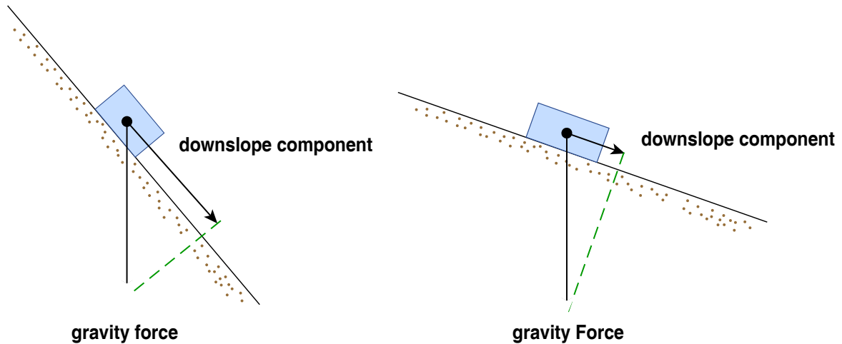
Figure 10-1. Resolving the force of gravity into a component in the downslope direction. The lengths of the arrows represent the magnitudes of the components of the gravity force. Left: a steep slope. Right: a gentle slope.
