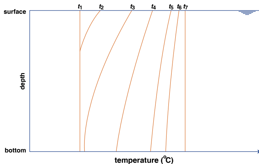
Figure by MIT OCW. Figure 6-11. Time series of temperature profiles during warming of your cold bath from the surface.
