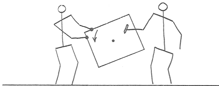
Figure 8-18. A simple way of demonstrating the Coriolis effect.
