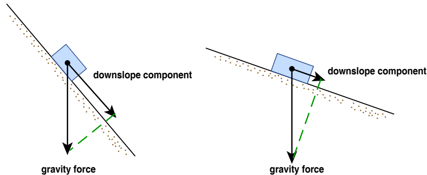
Figure 2-19. The downslope component of gravity acting on the layer of regolith. A) On a steep slope. B) On a less steep slope.
