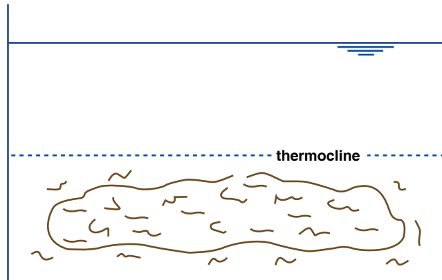
Figure 6-7. Near-independence of flow in the two layers.
