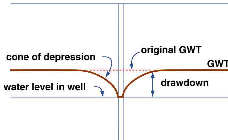
Figure 4-22. Geometry of the groundwater table around an active water well.
