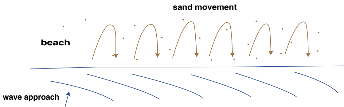
Figure 8-33. Beach drifting.
