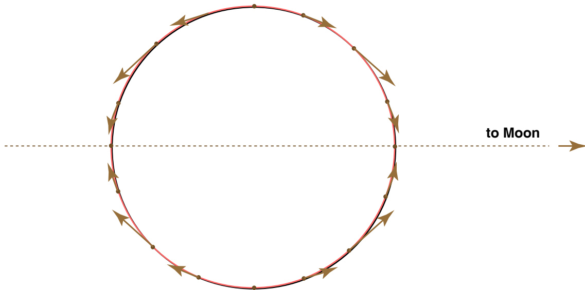
Figure 8-8. The horizontal component of the resultant tidal forces.
