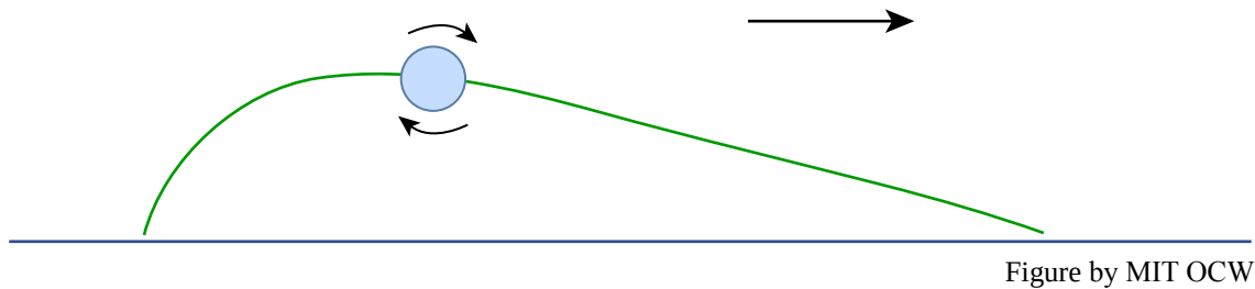
Figure 9-4. The sense of rotation of a saltating particle.
