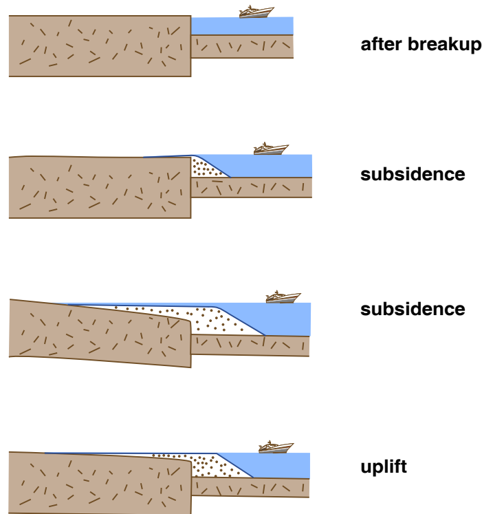
Figure 11-4. Recent geologic history of the Eastern Seaboard of North America.
