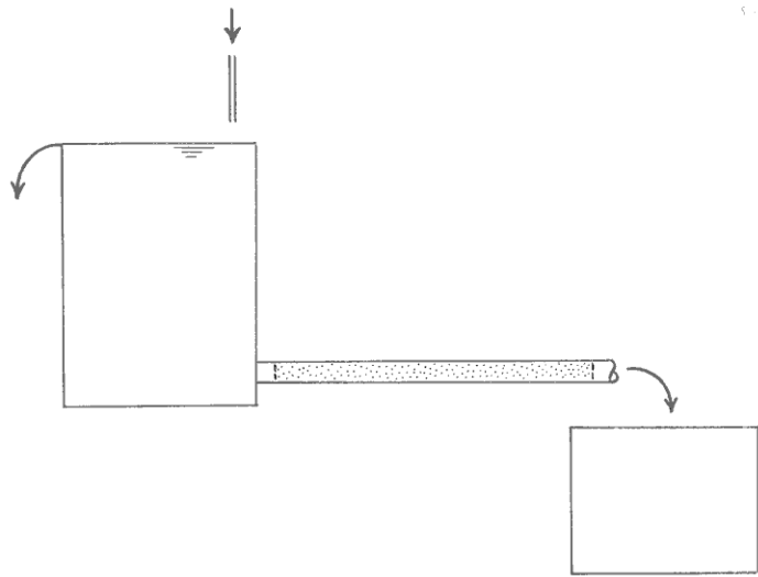
Figure 4-6. A home experiment on groundwater flow.
