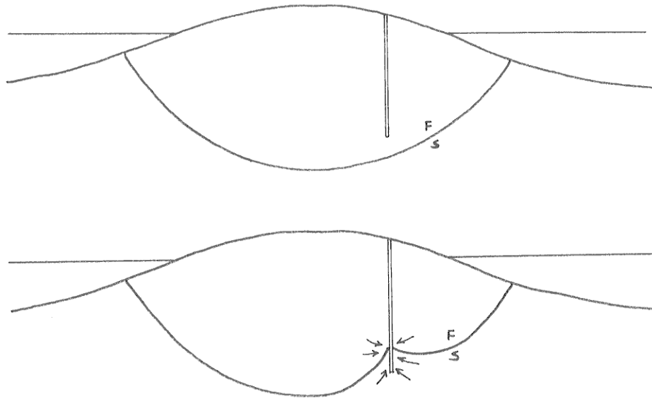
Figure 4-27. Effect of pumping on the position of the fresh-salt boundary beneath a coastal region.
