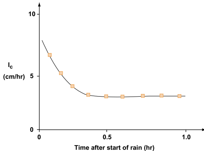
Figure 4-2. Plot of infiltration capacity against time for a given soil.
