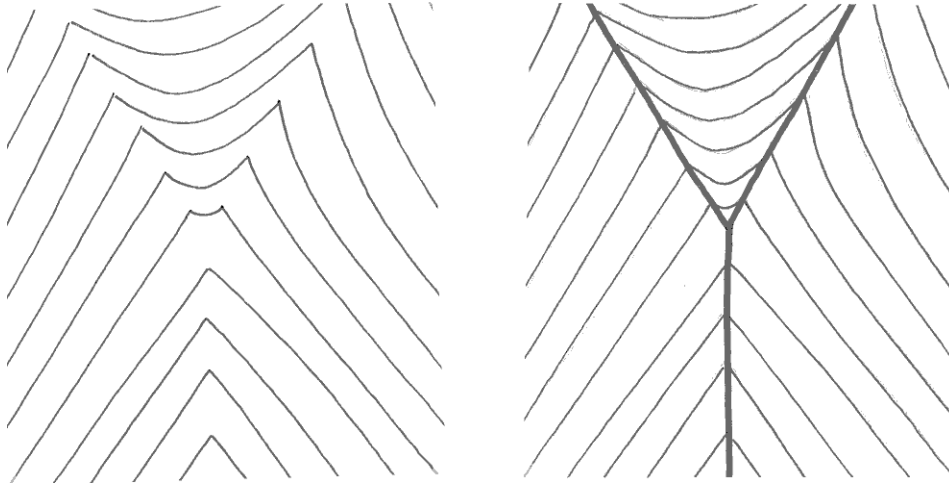
Figure 3-12. How you can locate the point of stream confluence by examining the “V”s of the contour lines.
