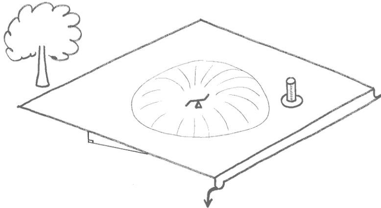
Figure 4-1. An experimental sprinkler plot for studying infiltration.
