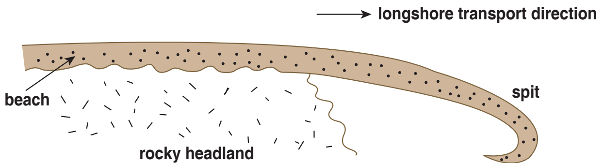
Figure 8-30. How sand piles up at the updrift sides of groins.
