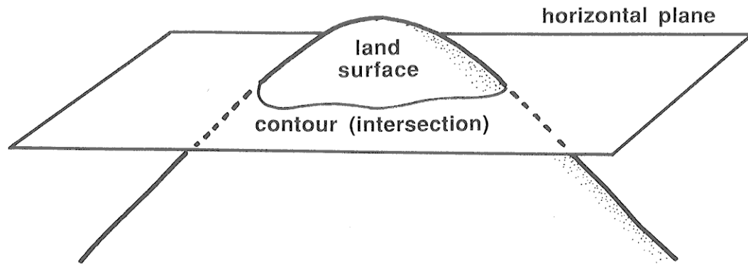
Figure 3-4. Viewing contours as the loci of horizontal planes with the land surface.
