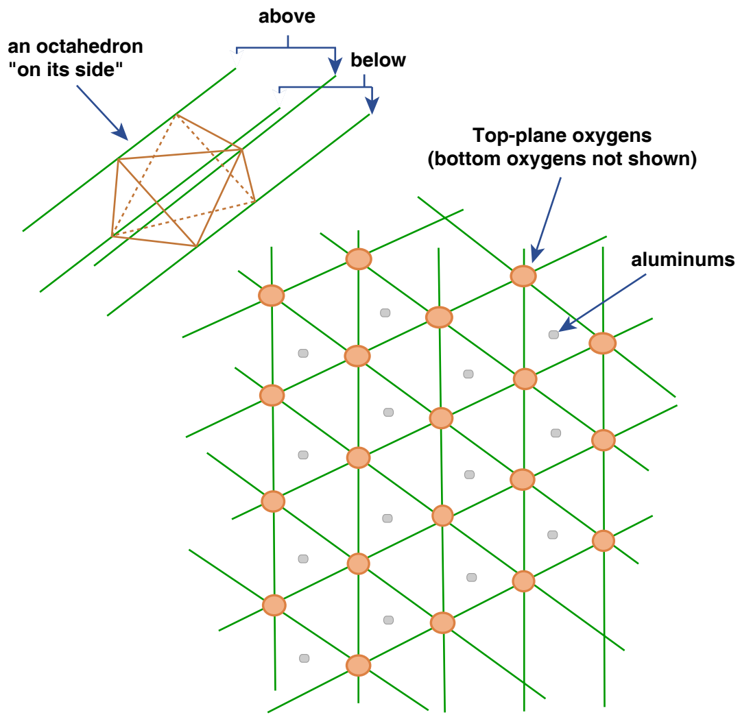
Figure 2-12. A more detailed view of the geometry of the octahedral sheet of clay-mineral structures.
