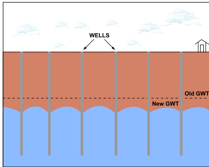
Figure 4-23. Geometry of the groundwater table in the vicinity of a number of closely spaced active water wells.
