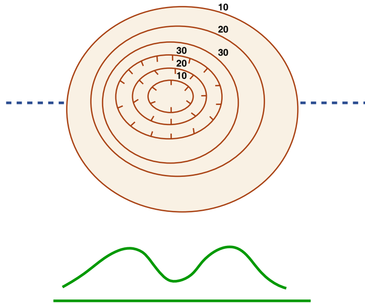
Figure 3-9. How contour lines represent depressions.
