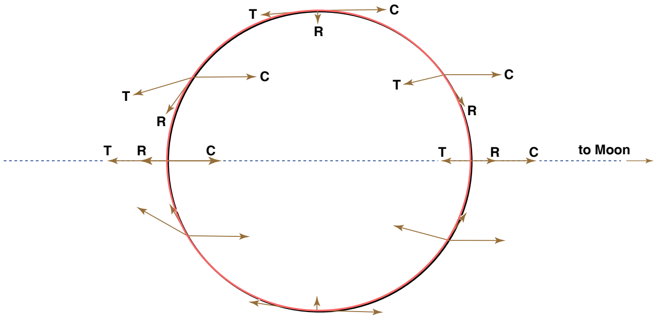
Figure 8-6. Tidal forces. T = gravitational force, C = centrifugal force, R = resultant force.
