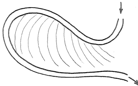
Figure 5-39. Meander scrolls.
