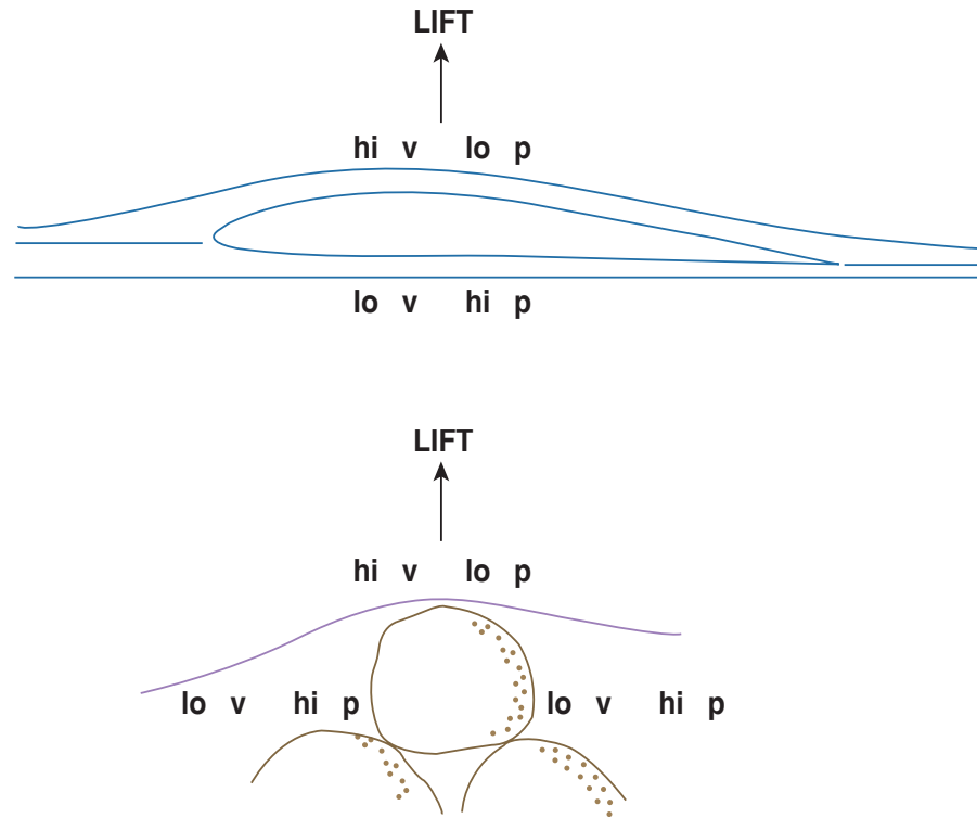
Figure 9-3. Aerodynamic lift forces. A) On an airplane wing. B) On a sediment particle.
