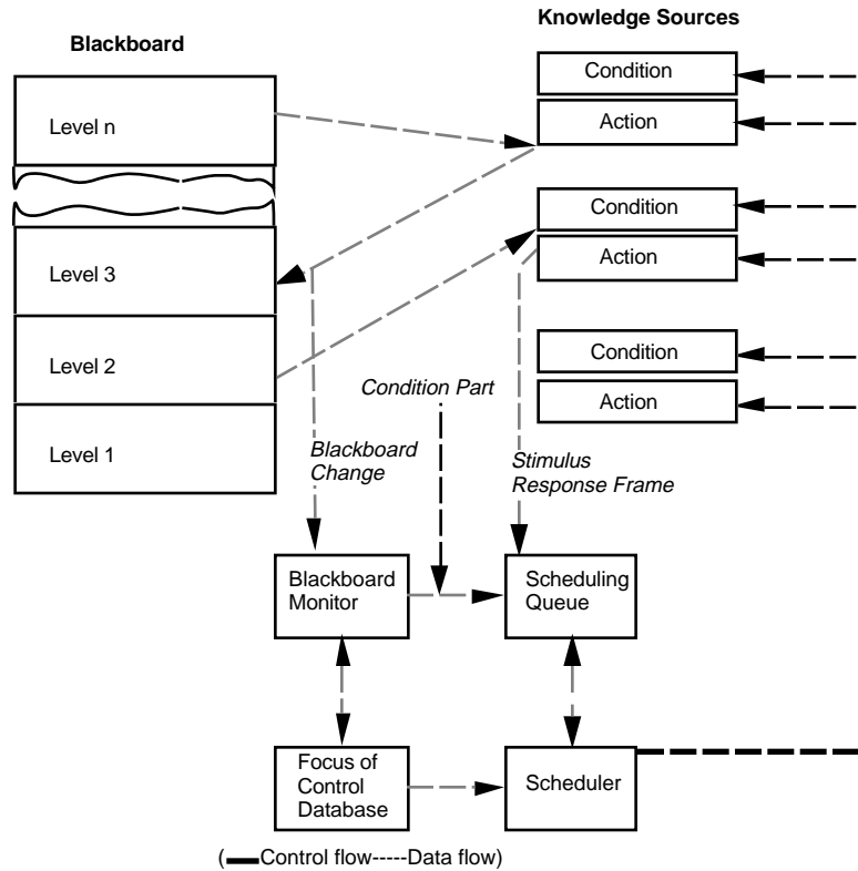
Figure 24: Hearsay-II
