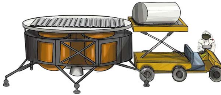
Figure 4-66. Evolved Payload Unloading Hardware
