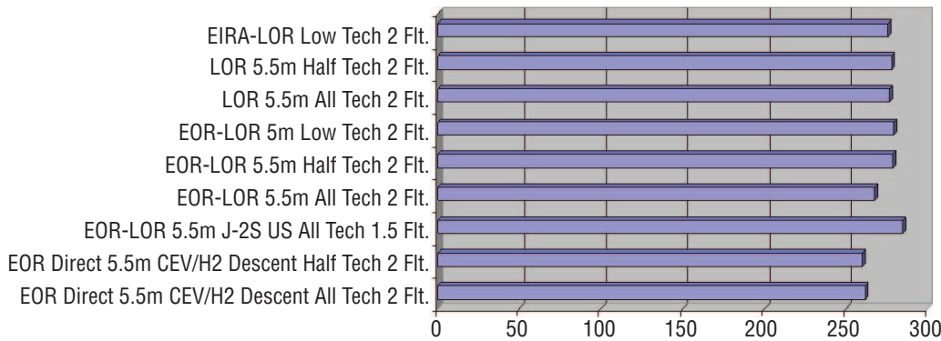
Figure 4-33. Analysis Cycle 2 Mission Mode Life Cycle Cost Comparison through 2025
