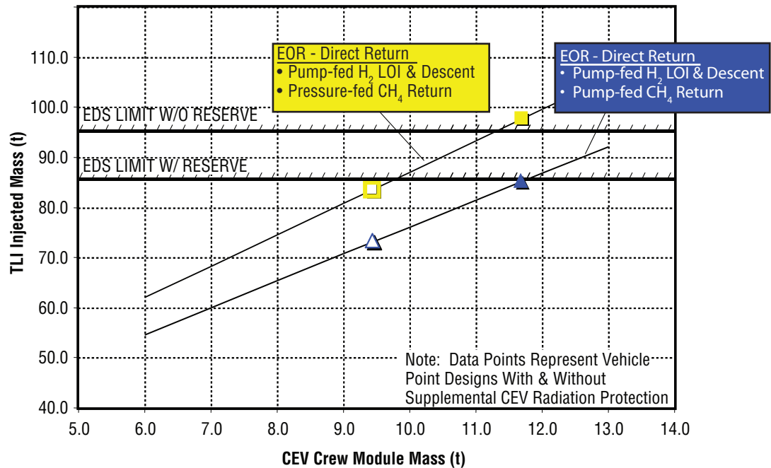
Figure 4-11. TLI Injected Mass versus Crew Compartment Mass, With and Without 5.0 g/cm 2 Supplemental Radiation Protection
