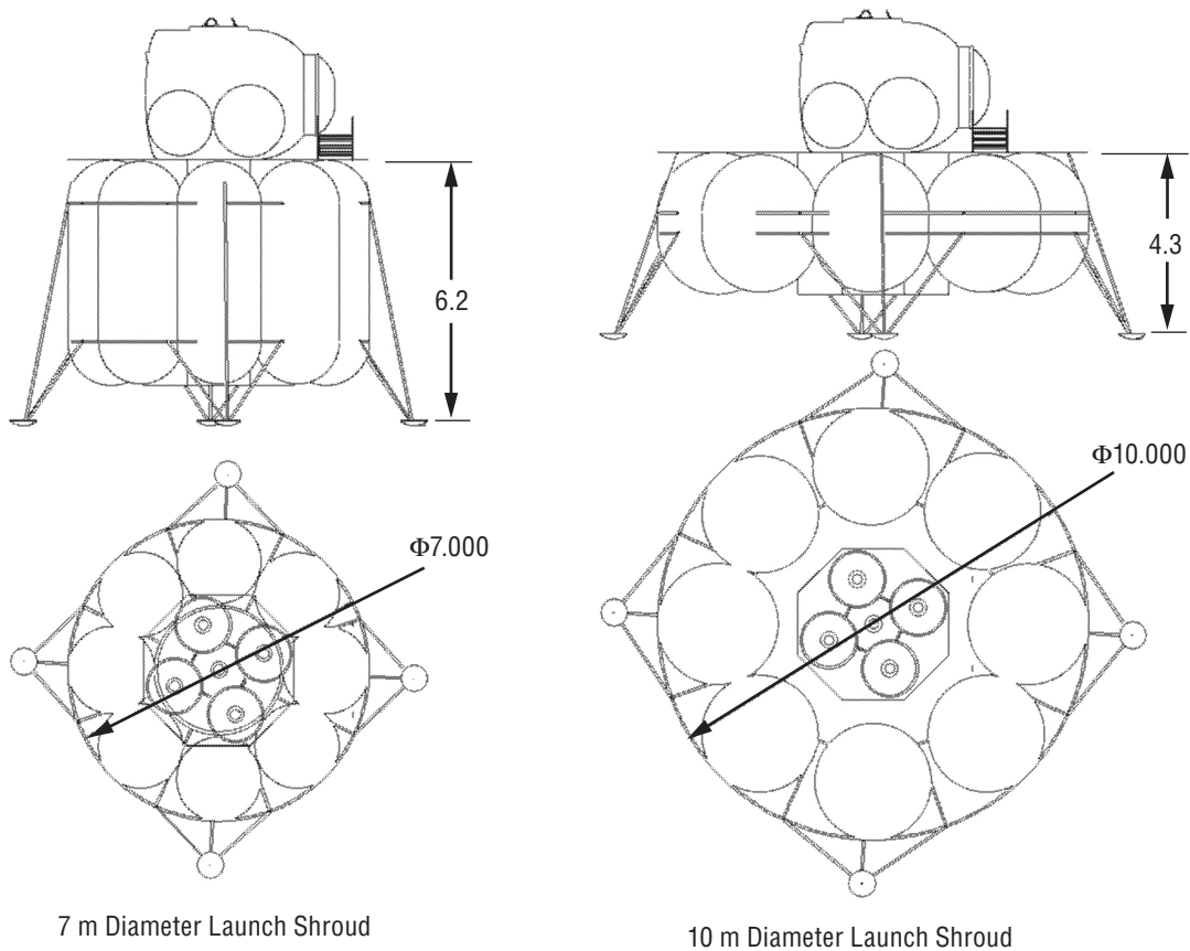
Figure 4-44. Launch Shroud Diameter Influence on LSAM Tank Configuration
