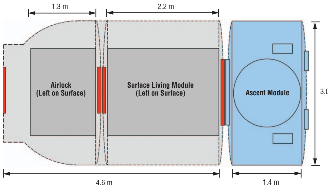
Figure 4-45. LSAM Minimized Crew Module Vehicle Configuration
