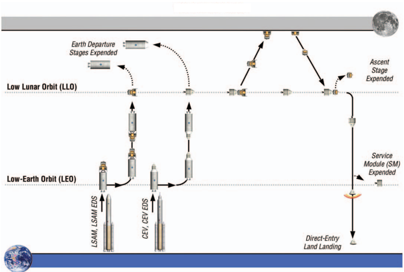
Figure 4-3. ESAS Initial Reference Architecture
