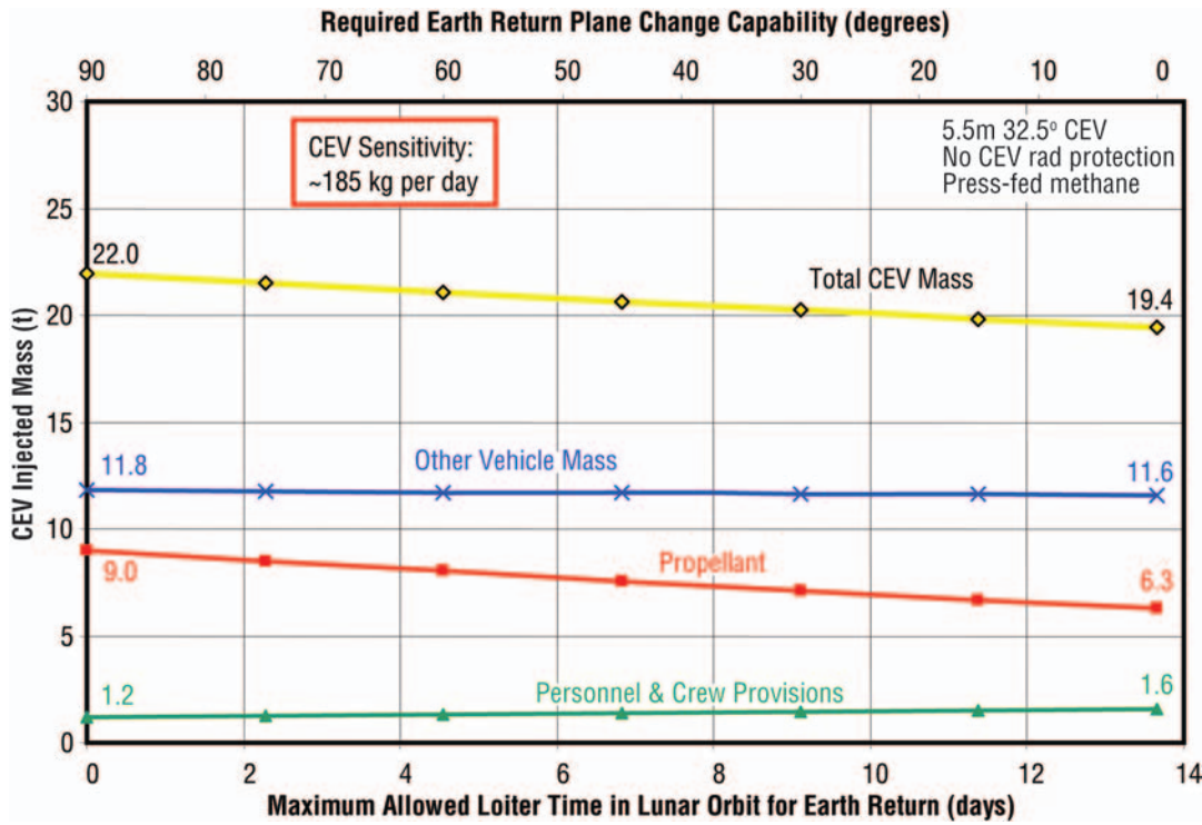
Figure 4-40. CEV Anytime Return Performance
