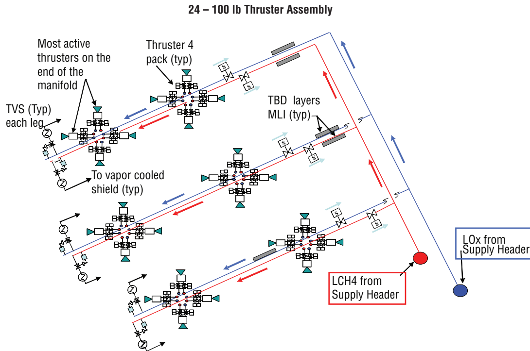
Figure 4-16. RCS Manifolds
