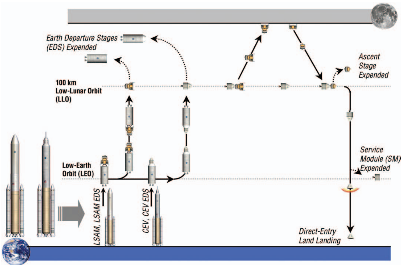
Figure 4-5. EIRA Architecture Illustration (Analysis Cycle 1)
