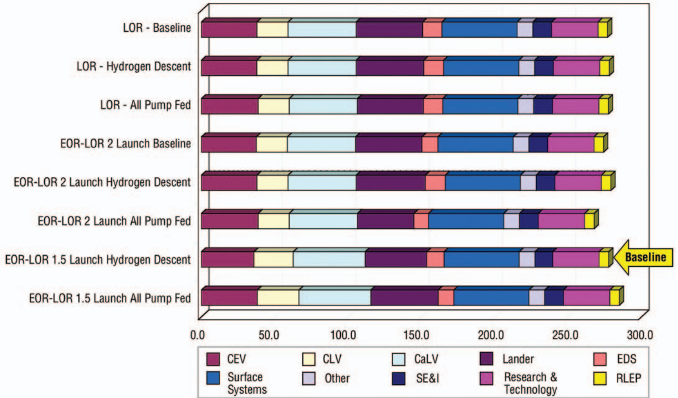
Figure 4-56. Mission Mode Life Cycle Costs Through 2025
