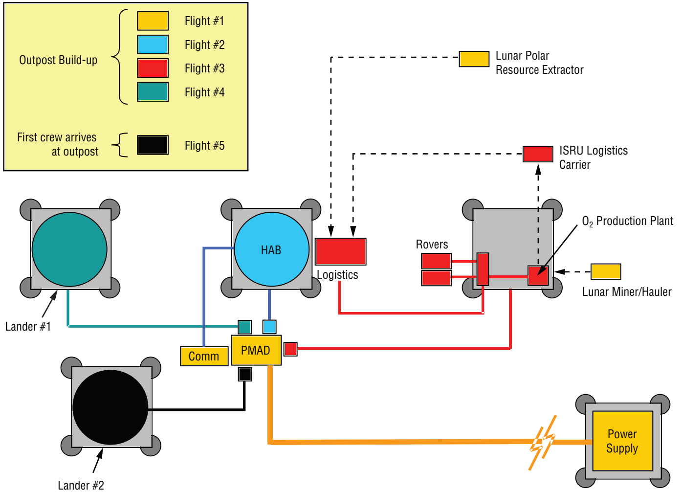
Figure 4-64. Core Outpost Schematic
