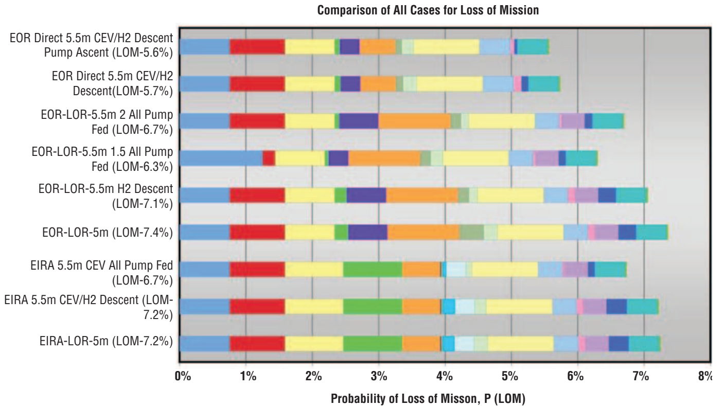
Figure 4-34. Analysis Cycle 2: Loss of Mission Comparison
