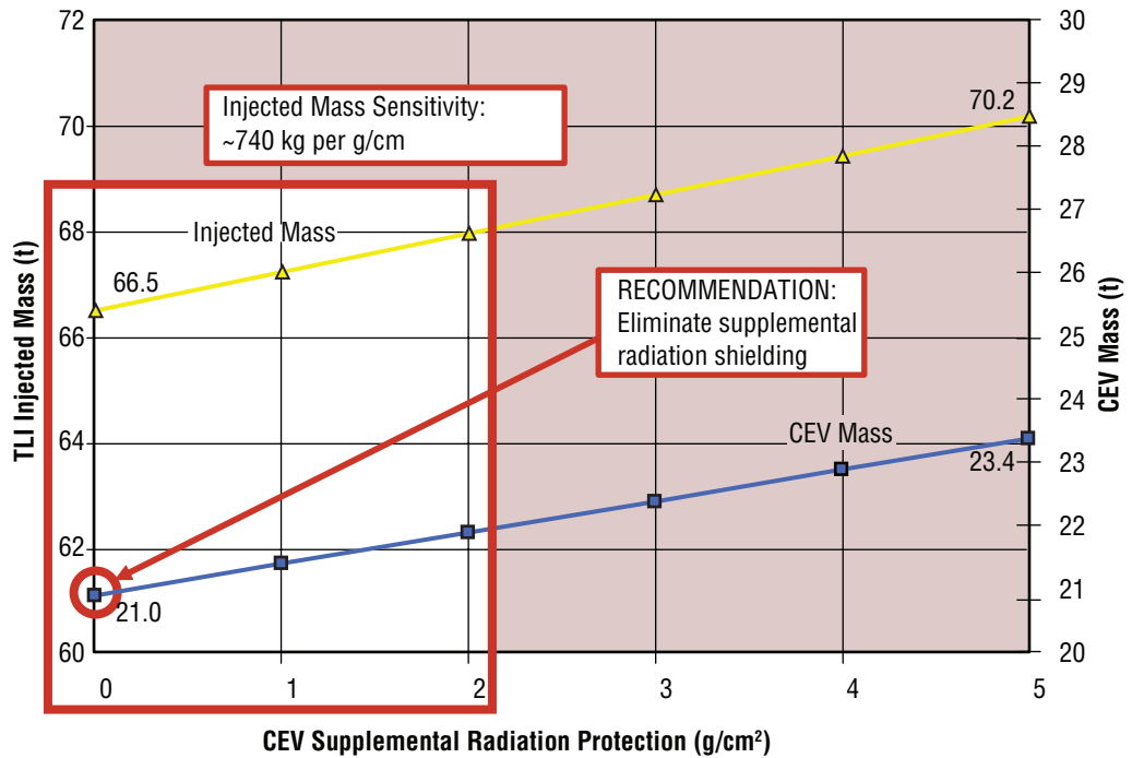
Figure 4-36. 1.5 Launch EOR-LOR Sensitivity to CEV Radiation Protection
