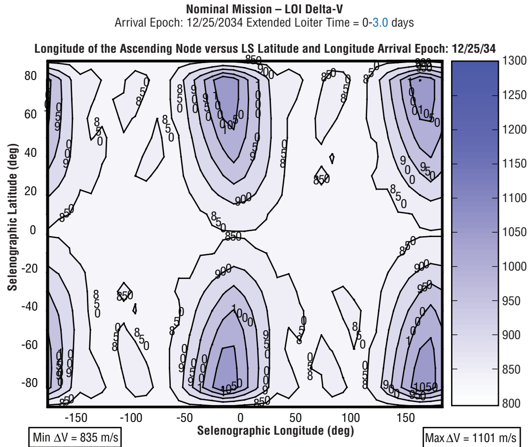
Figure 4-39. Global LOI Delta-V Map, 3 Day Loiter Time
