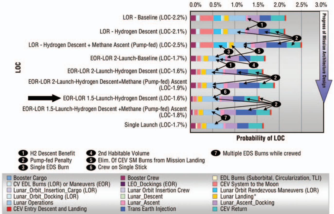
Figure 4-54. Loss of Crew Comparison
