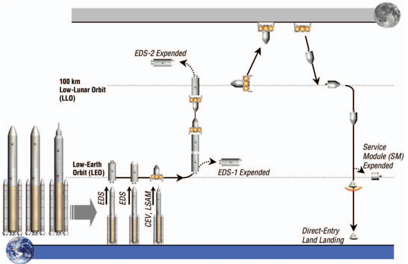
Figure 4-7. EOR-Direct Architecture Illustration (Analysis Cycle 1)
