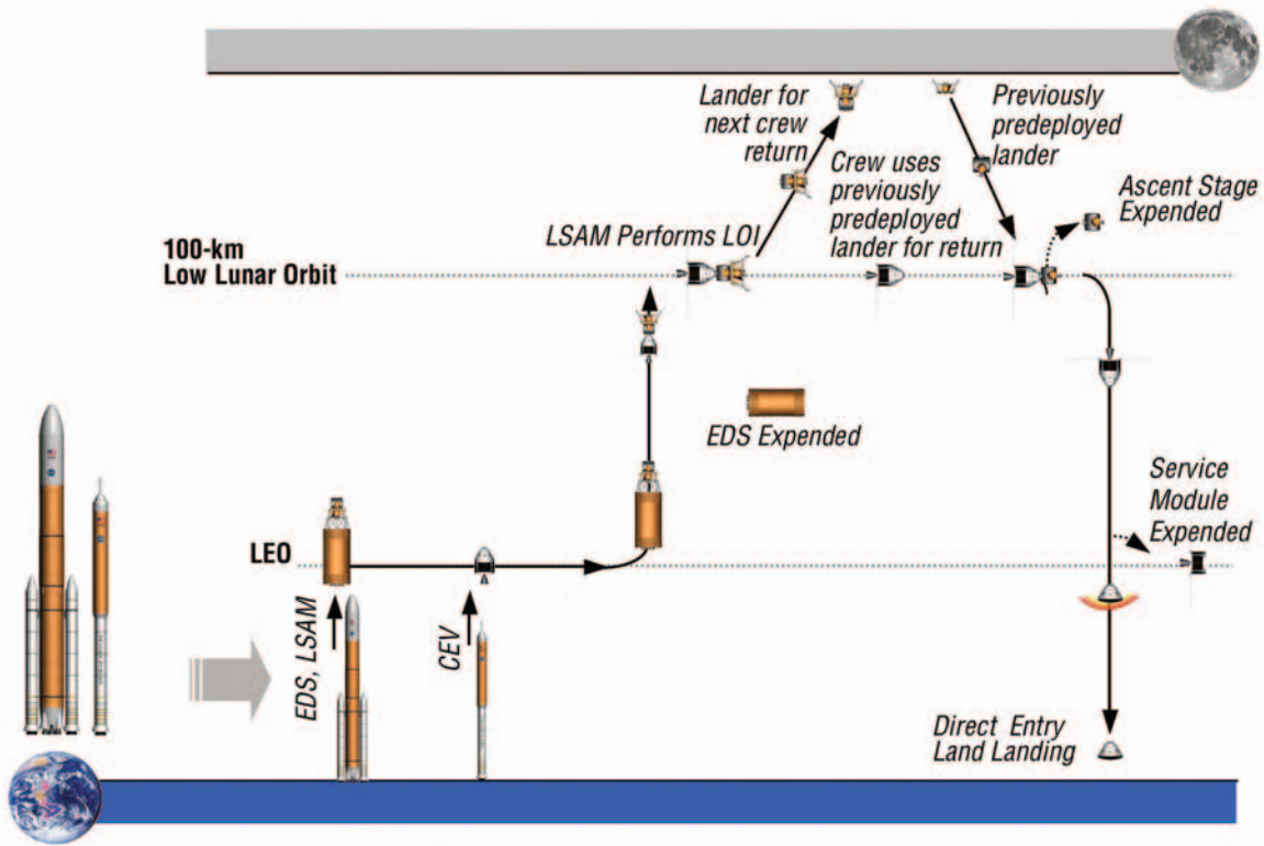
Figure 2-7 Lunar Outpost Crew and Cargo Transportation DRM
