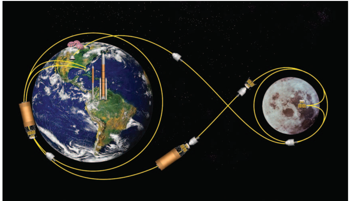
Figure 4-58. EOR-LOR "1.5 Launch" Lunar Mission Architecture
