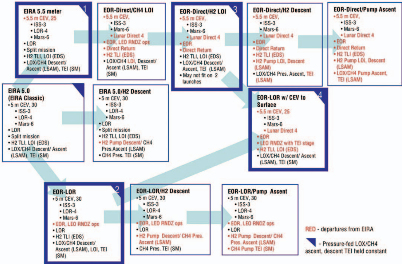
Figure 4-4. Analysis Cycle 1 Mission Architecture Flow
