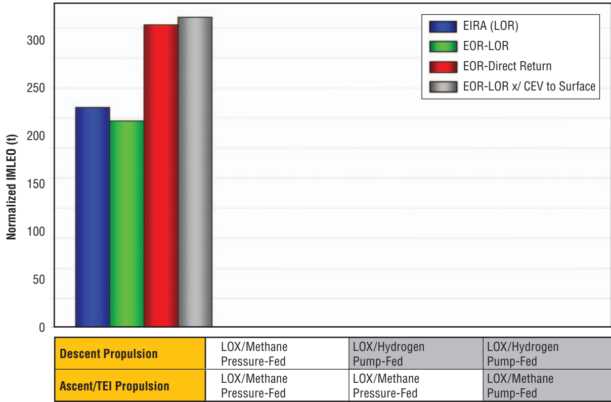
Figure 4-9. Analysis Cycle 1 Normalized IMLEO Comparison
