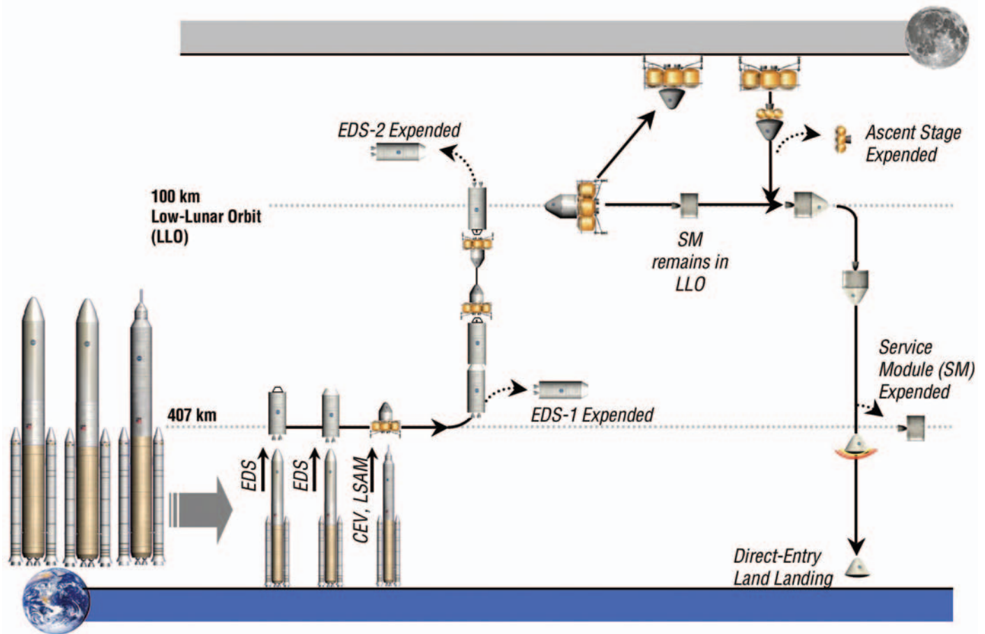
Figure 4-8. EOR-LOR with CEV-to-Surface Architecture Illustration (Analysis Cycle 1)
