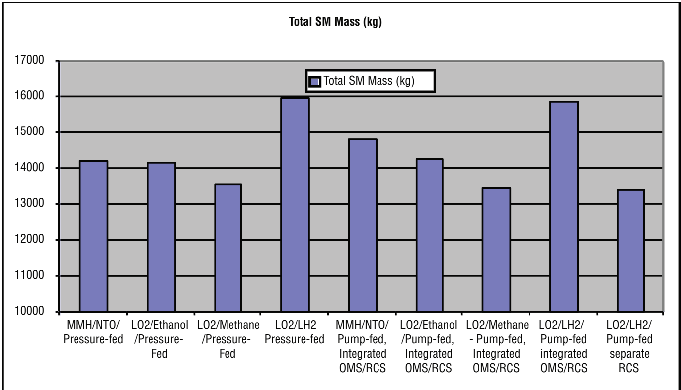
Figure 4-12. Total SM Mass
