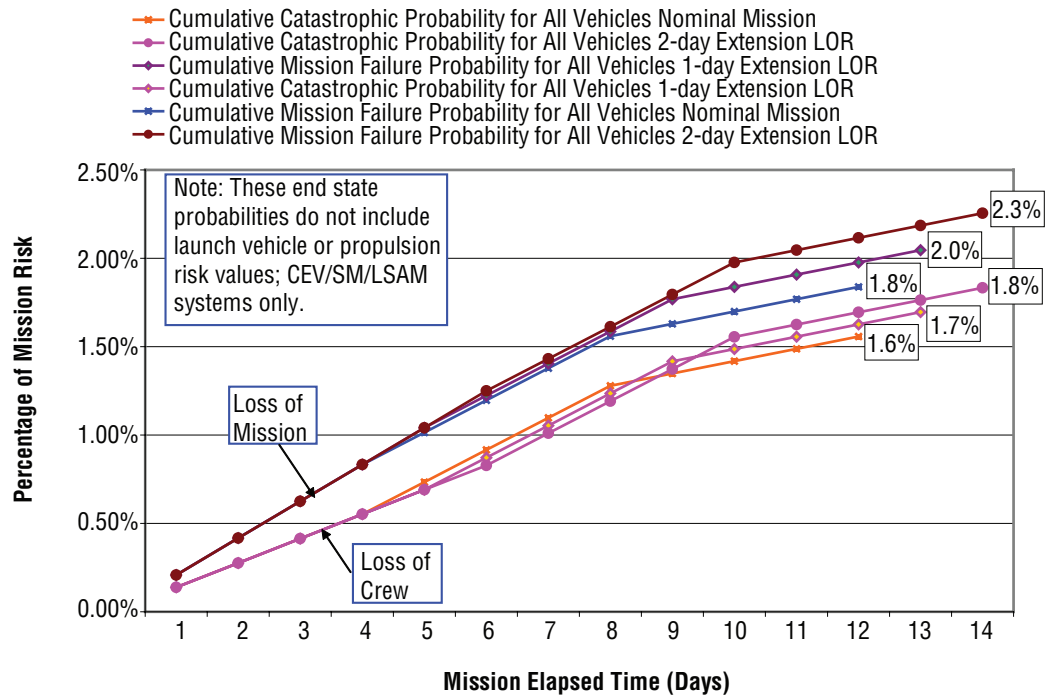
Figure 4-41. Delta P(LOC) and P(LOM) for Extending Orbital Loiter Prior to Lunar Descent
