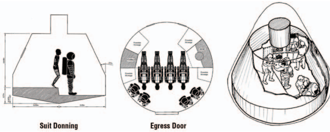
Figure 4-25. Single-Volume EOR-Direct Return Initial Conceptual CEV Layouts
