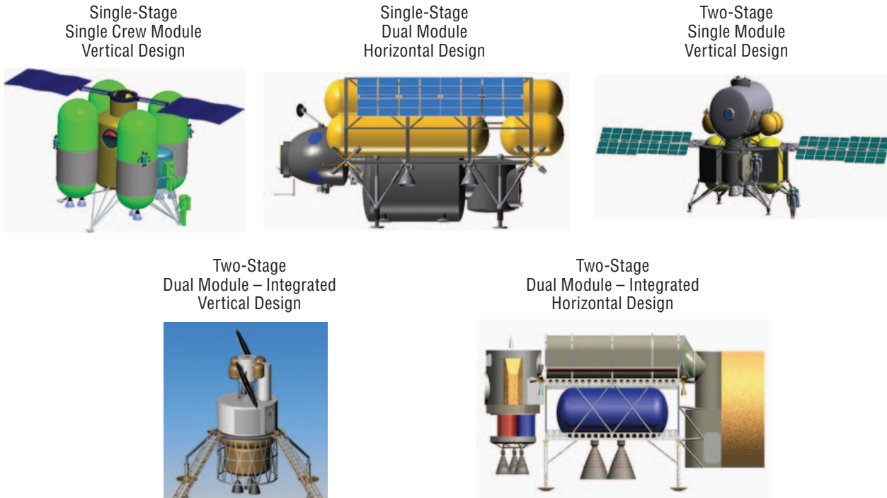
Figure 4-42. Initial LSAM Configurations
