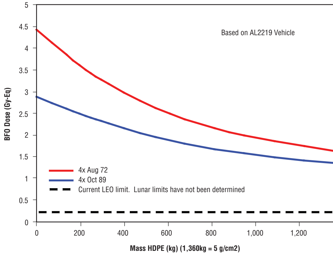
Figure 4-10. Mass of HDPE
