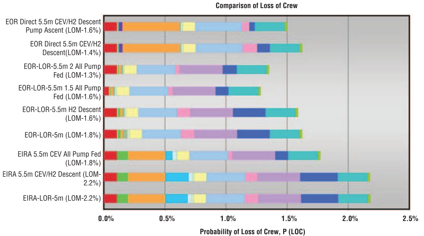
Figure 4-35. Analysis Cycle 2: Loss of Crew Comparison
