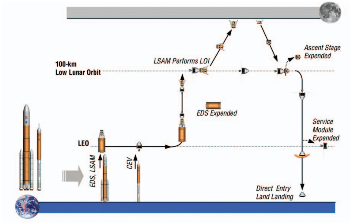
Figure 2-5. Lunar Sortie Crew and Cargo DRM
