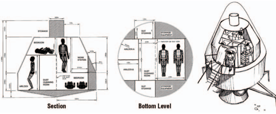
Figure 4-24. Single-Volume CEV Study Design Layouts
