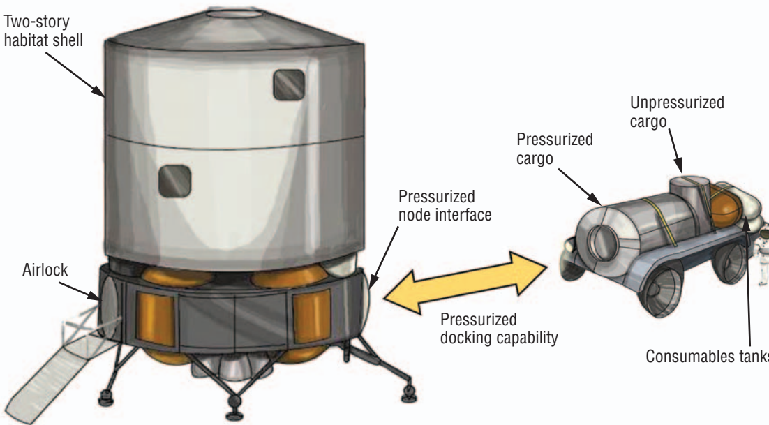
Figure 4-67. Habitat Mass Partitioning Strategy
