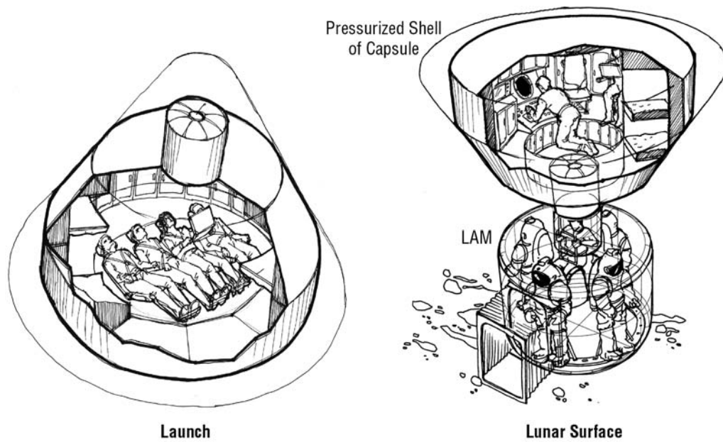
Figure 4-23. Split-Volume EOR-Direct Return CEV + Airlock Module Layout by Flight Phases
