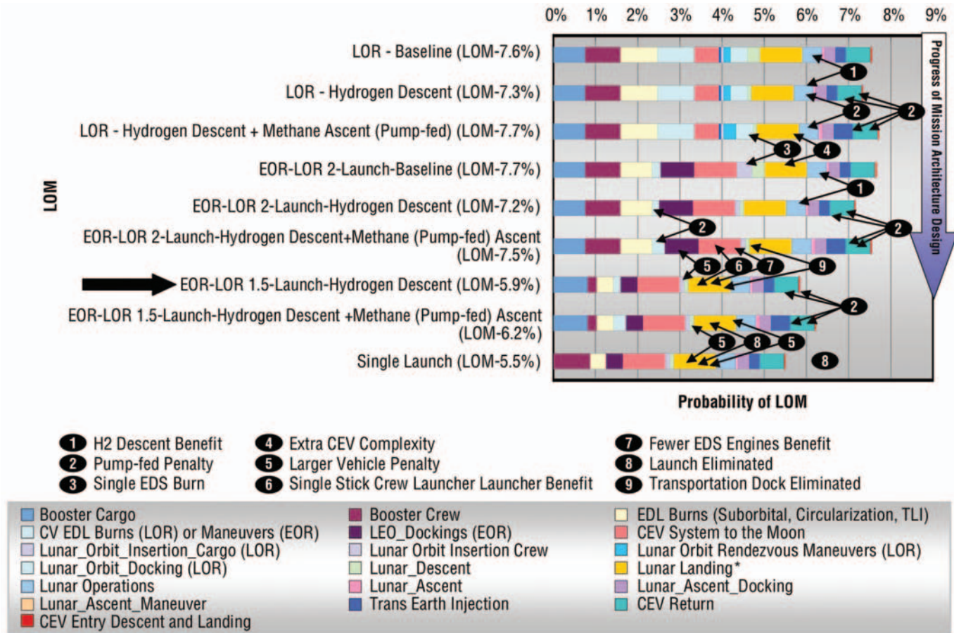
Figure 4-55. Loss of Mission Comparison
