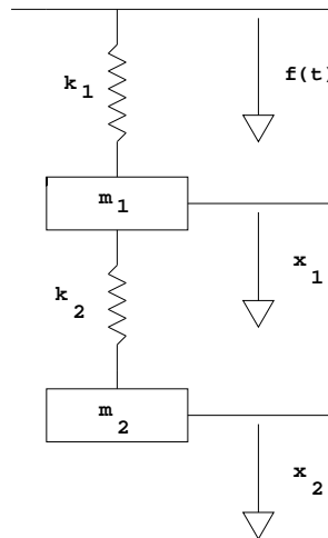
FIGURE 16. Two spring system
