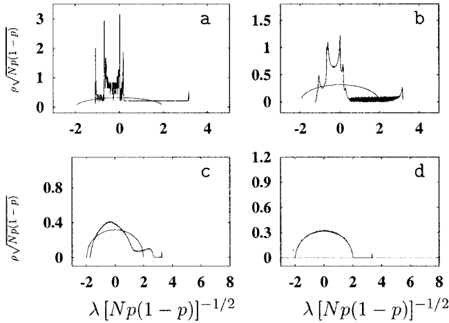
FIG. 3. Spectral densities of small-world graphs using the complete spectra. The solid line shows the semicircular distribution for comparison. (a) Spectral density of the regular ring graph created from the small-world model with p_r=0 , k=10 , and N=1000 . (b) For p_r=0.01 , the average spectral density of small-world graphs contains sharp maxima, which are the “blurred” remnants of the singularities of the p_r=0 case. Topologically, this means that the graph is still almost regular, but it contains a small number of impurities. In other words, after a small perturbation, the system is no longer degenerate. (c) The average spectral density computed for the p_r=0.3 case shows that the third moment of \rho(\lambda) is preserved even for very high values of p_r , where there is already no sign of any blurred singularity (i.e., regular structure). This means that even though all remaining regular islands have been destroyed already, triangles are still dominant . (d) If p_r=1 , then the spectral density of the small-world graph converges to a semicircle. In (b), (c), and (d), 1000 different graphs with N=1000 and k=10 were used for averaging.
