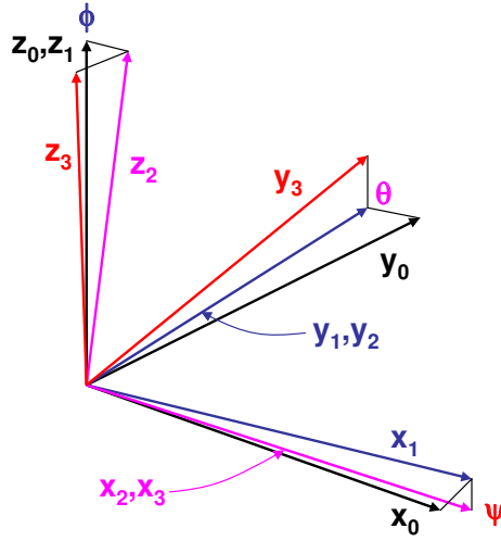
Figure 1: Successive application of three Euler angles transforms the original coordinate frame into an arbitrary orientation.
