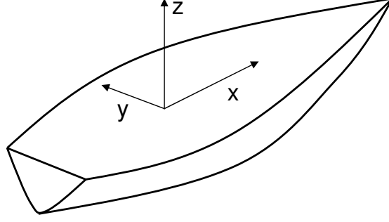
Figure 2: Convention for the body-referenced coordinate system on a vehicle: x is forward, y is sway to the left, and z is heave upwards. Looking forward from the vehicle "helm," roll about the x axis is positive counterclockwise, pitch about the y -axis is positive bow-down, and yaw about the z -axis is positive turning left.
