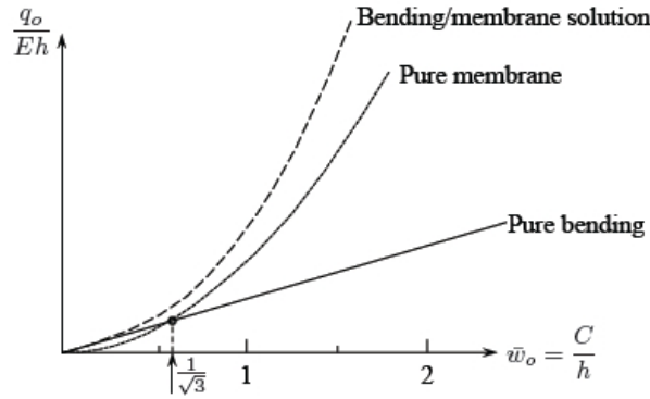
Figure 6.3: Comparison of a bending and membrane solution for a beam.
