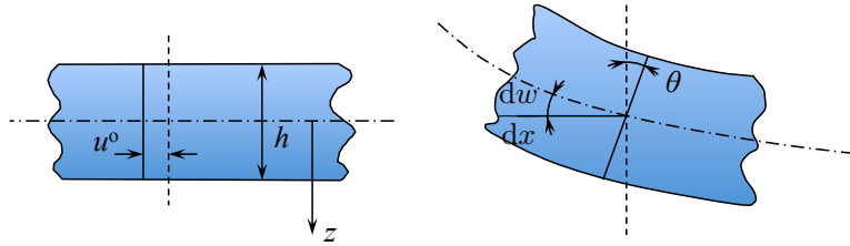
Figure 2.17: Linear displacement field through the thickness of the beams.
