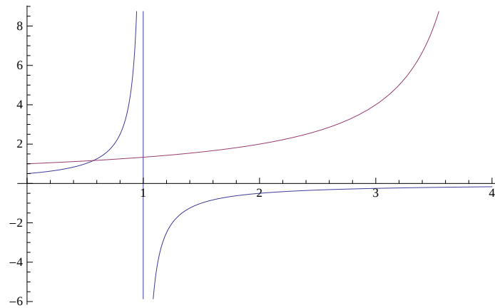
Figure 9.14: The deformation amplitudes B_1 , B_2 vs. load \bar{P} curves, for the case A_1 = 0.5 .
