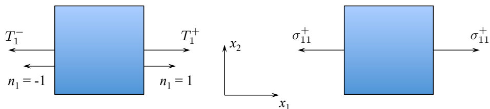
Figure 3.10: Explanation of the sign convention of the stress tensor.
