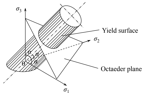
Figure 12.6: Representation of the von Mises yield condition in the space of principal stresses.
