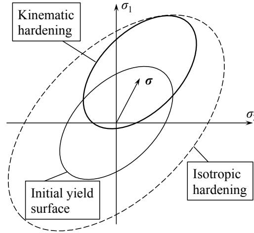
Figure 12.8: Comparison of the isotropic and kinematic hardening under plane stress.
