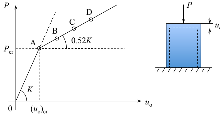
Figure 11.14: Pre and post-buckling response of a plate.
