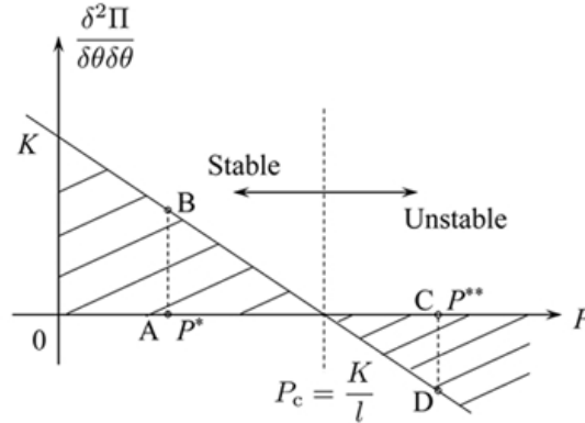
Figure 9.2: Stable and unstable range in column buckling.
