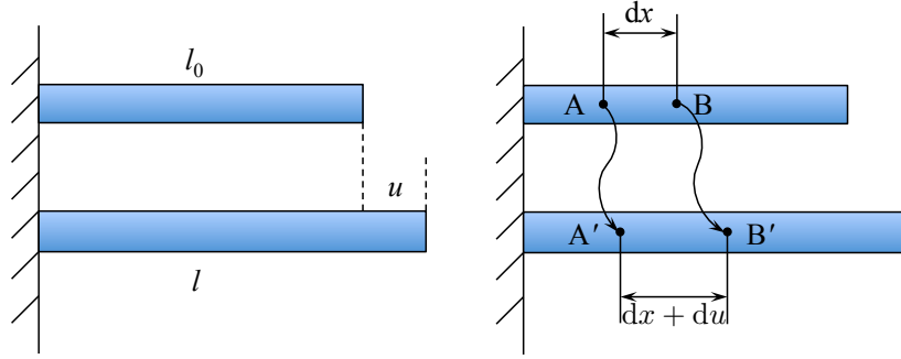
Figure 2.2: Undeformed and deformed element in the homogenous and inhomogeneous strain field in the bar.
