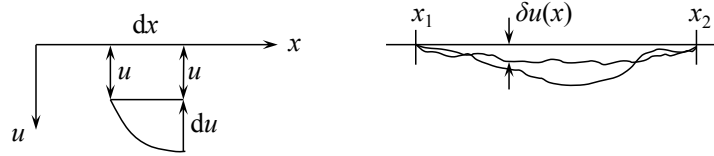
Figure 3.12: The local increment \delta u over the infinitesimal length dx and the global small (virtual) displacement from the equilibrium configuration satisfying kinematic boundary conditions.
