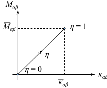
Figure 4.9: The straight loading path in the 3-dimensional space of bending moments..
