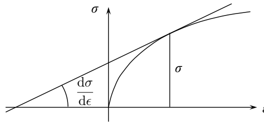
Figure 9.11: The construction of Considère' who was the first to derive Eq. (9.66).
