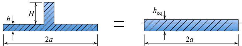
Figure 7.11: Geometry of plate/beam combination and the equivalent thickness plate.
