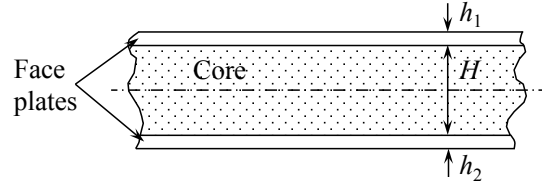
Figure 7.3: There are two materials and three different thicknesses in sandwich plates.
