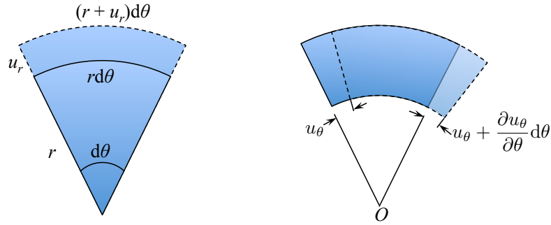
Figure 2.9: Two deformation modes responsible for the circumferential (hoop) strain.
