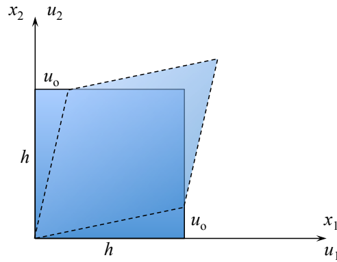
Figure 2.5: Imposing constant deformative gradients.
