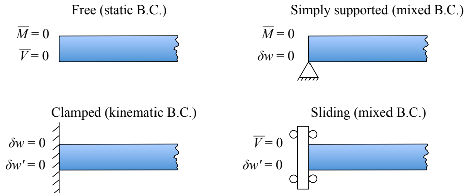
Figure 3.19: Boundary conditions in the axial direction.
