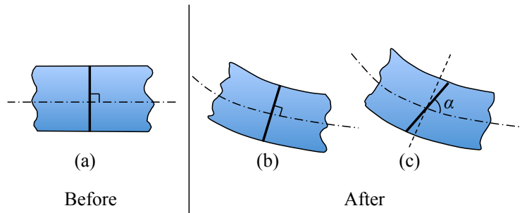
Figure 2.16: Testing the normal-remains-normal hypothesis.
