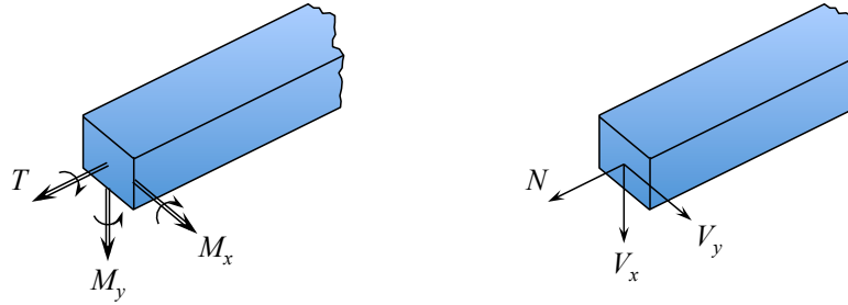
Figure 3.15: Imagine short shafts rotating a rigid slice of the beam. These are components of the bending moment vector.
