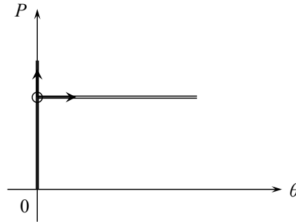
Figure 9.4: Two equilibrium paths intersect at the bifurcation point.
