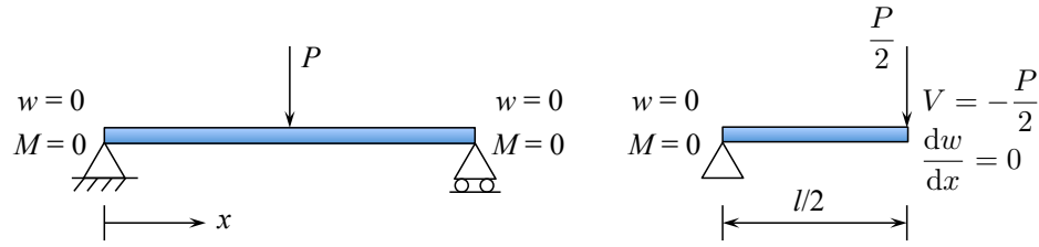
Figure 5.6: Symmetric loading of a beam by a concentrated force.
