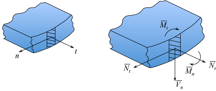
Figure 3.25: Local coordinate system at the plate edge with applied generalized forces.
