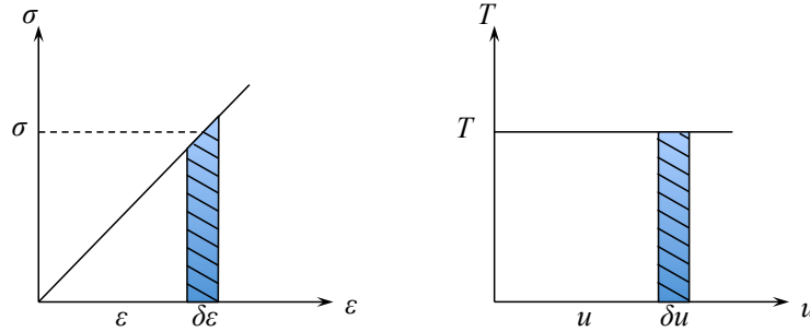
Figure 3.14: Incremental internal and external energies.
