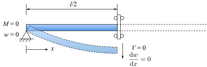
Figure 5.4: Simply-supported plate with symmetry boundary conditions.
