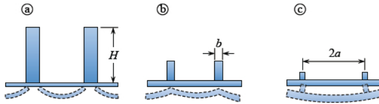
Figure 7.10: Heavy, intermediate and light stiffeners.
