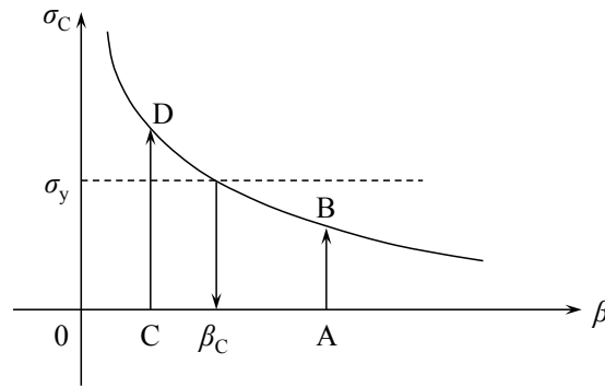
Figure 9.12: A hyperbolic dependence of the buckling stress on the slenderness ratio.
