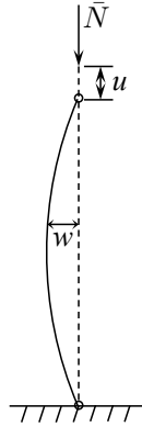
Figure 9.6: Initial and deformed elastic column.
