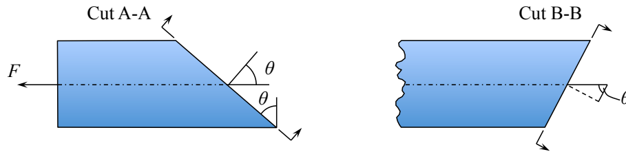
Figure 3.3: Normal and tangential forces acting on the slant section of the bar.
