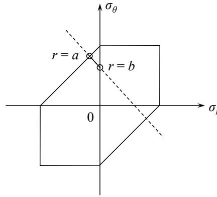
Figure 12.16: The stress profile across the thickness of the cylinder.
