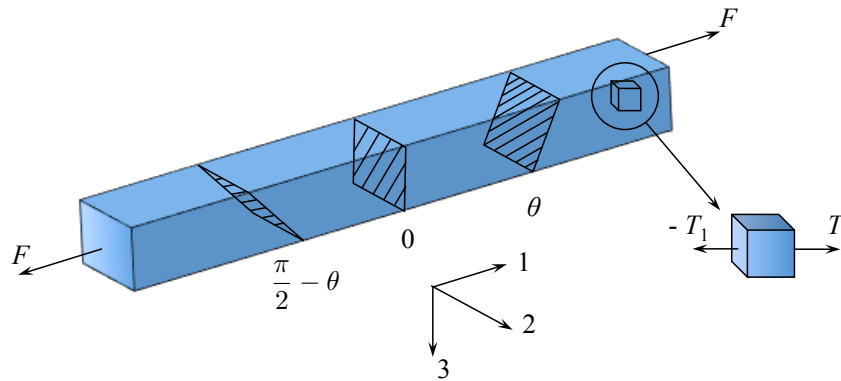
Figure 3.1: A long bar with three different cuts at \theta , \theta = 0 and \pi/2 - \theta .
