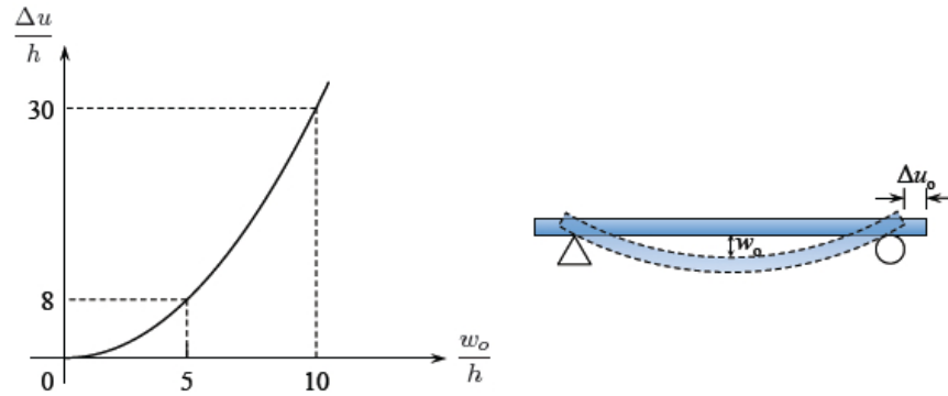
Figure 6.2: Sliding of a beam from the roller support.
