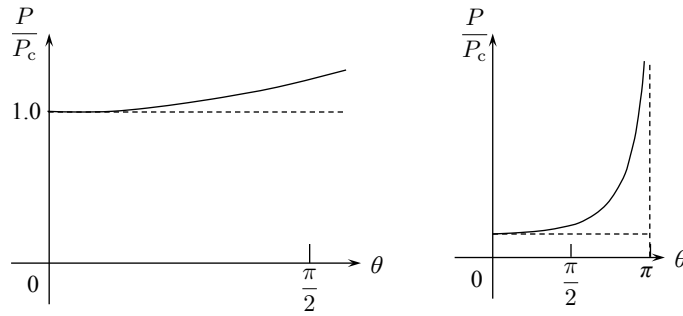
Figure 9.5: Plot of the secondary equilibrium path.
