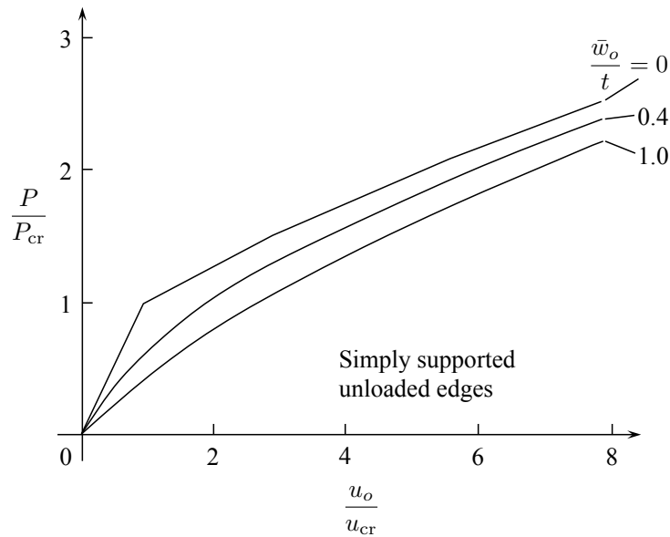
Figure 11.17: Load-displacement curves for imperfect simply supported plates.
