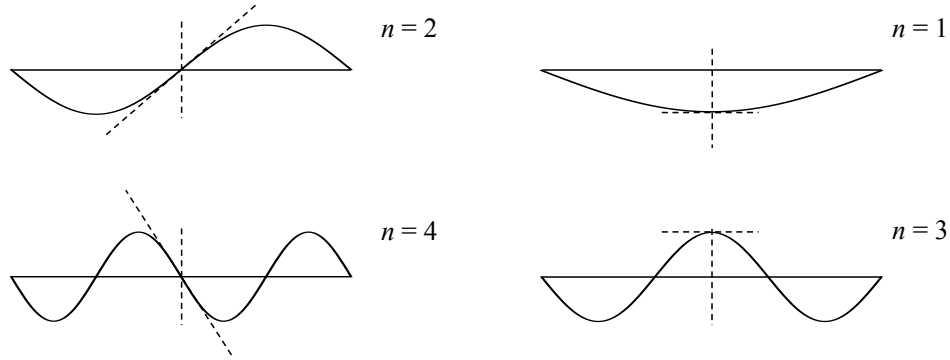
Figure 8.5: Asymmetric modes do not satisfy boundary condition w'(x = \frac{l}{2}) = 0 at the center of the beam.
