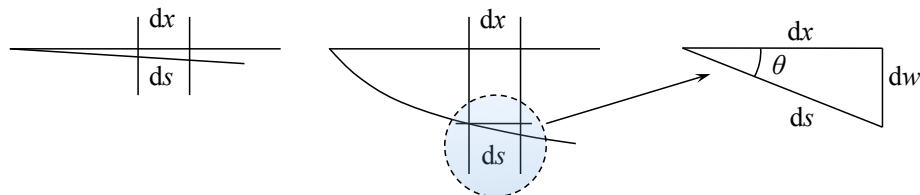
Figure 2.21: Change of length of the beam axis produced by rotation.
