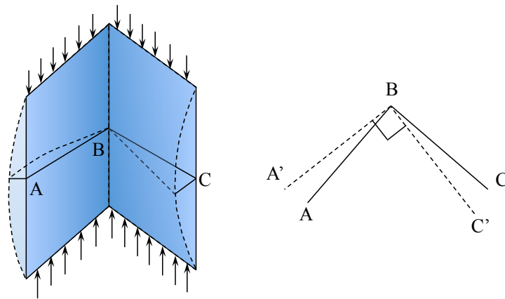
Figure 11.5: Buckling mode of an angle element.
