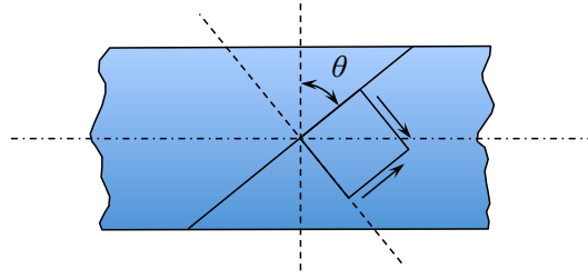
Figure 3.4: The volume element with surface traction acting on two adjacent facets.
