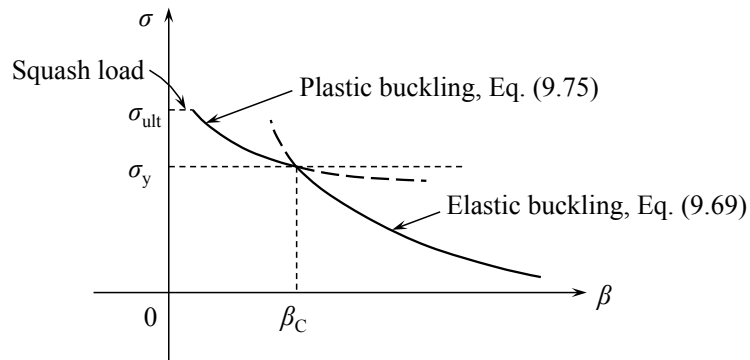
Figure 9.13: Range of elastic and plastic buckling.
