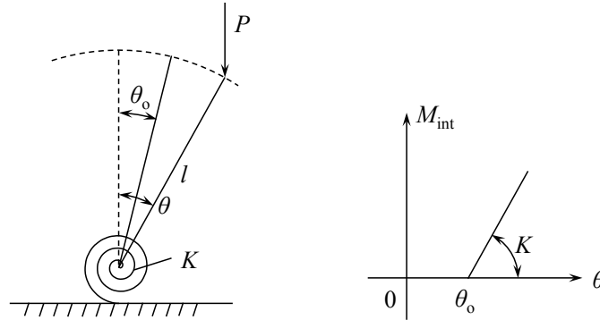
Figure 9.7: The initial inclination angle \theta_o is a measure of structural imperfection.
