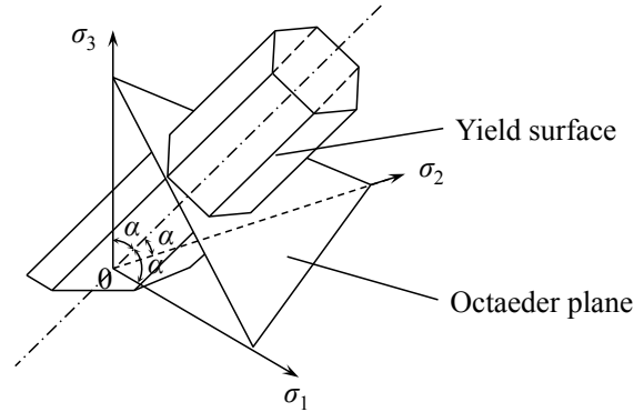
Figure 12.11: Representation of the Tresca yield condition in the space of principal stresses.
