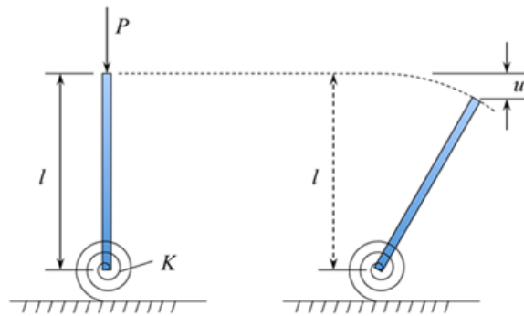
Figure 9.3: A discrete Euler column in the undeformed and deformed configuration.
