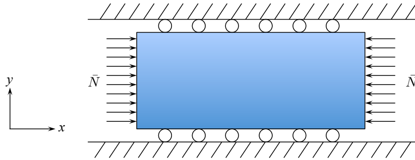
Figure 11.3: Constrained compression of the plate.
