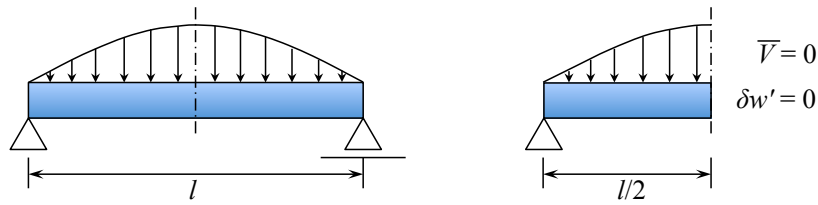
Figure 3.21: Shear force V and rotation angle \delta w' vanishes at the symmetry plane.
