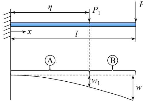
Figure 8.12: Cantilever beam loaded by two point forces.
