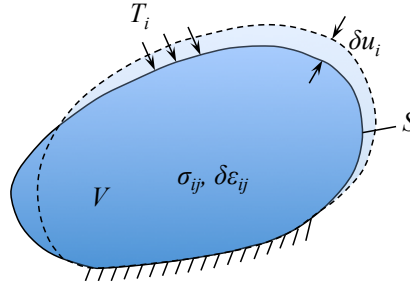
Figure 3.13: The 3-D potato (body) subjected to stress and displacement boundary condition develops internal stresses and incremental displacements.
