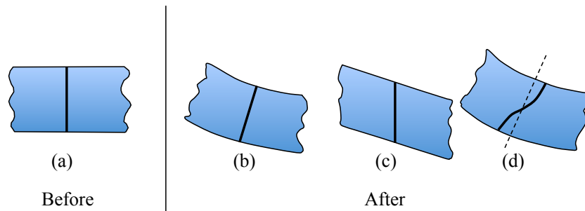
Figure 2.15: Flat (b) and (c) and warped (d) cross-sections after deformations.
