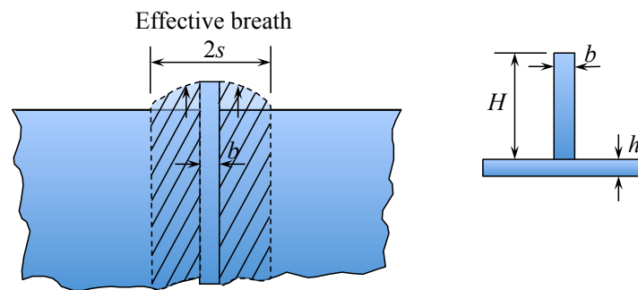
Figure 7.15: In-plane shear induced by the stiffener is restricted to an immediate vicinity of the stiffener.
