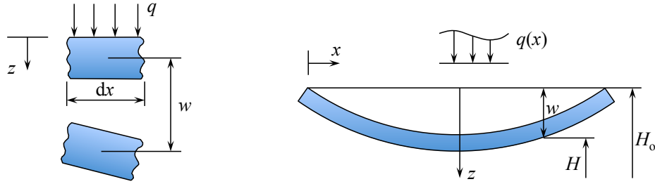
Figure 8.2: Potential energy of a beam element and the entire beam.
