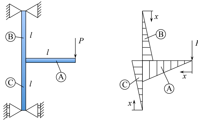
Figure 8.9: Statically determined system and bending moment distribution.
