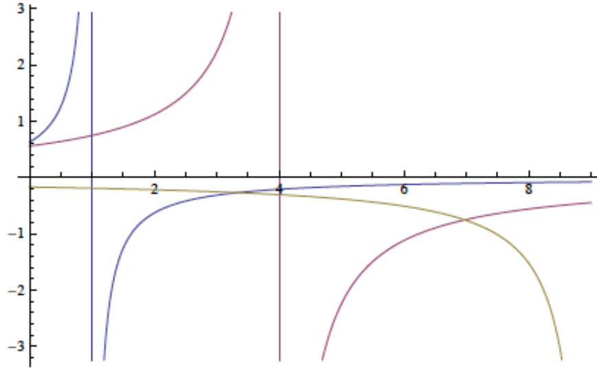
Figure 9.17: The deformation amplitudes of the first three modes vs. load \bar{P} curves, for the imperfection shape described by Eqn. 9.92.
