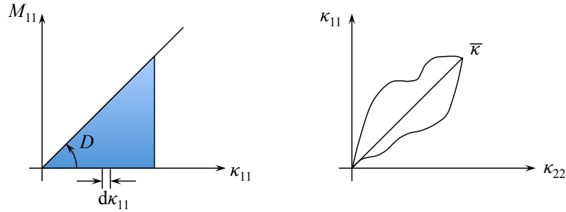
Figure 4.8: In one dimension the energy density is the area under the linear moment-curvature plot. In the multi-axial case the final value can be reached along the straight or nonlinear path.
