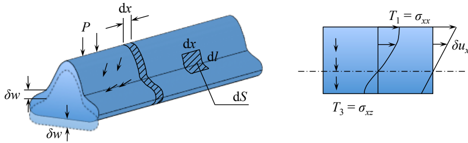
Figure 3.18: The outer surface of the beam consists of two parts: the lateral surface S_L on which the surface traction are acting and the end cuts A .
