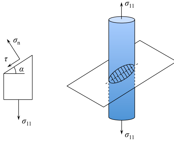
Figure 12.10: Shear and normal stresses at an arbitrary cut.
