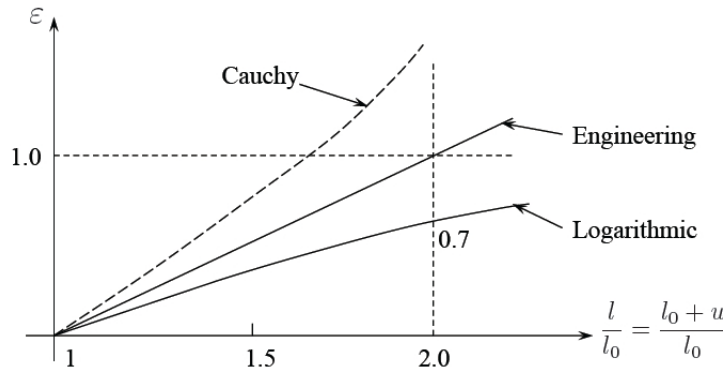
Figure 2.1: Comparison of three definitions of the uniaxial strain.
