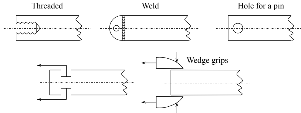
Figure 3.2: How to apply tension to the end of a bar.
