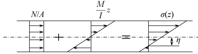
Figure 4.5: Linear distribution of stresses along the height of the beam.
