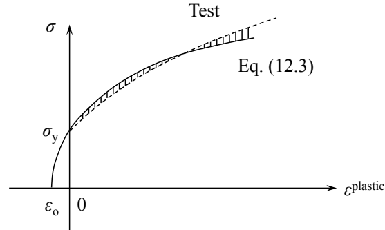
Figure 12.2: The experimentally measured stress-strain curve and the fit by the swift law.
