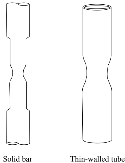
Figure 9.10: Necking in a solid section bar and thin-walled tube under tension.
