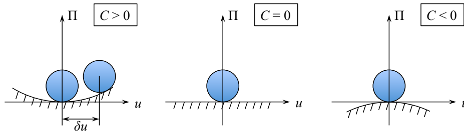
Figure 9.1: Illustration of stable, neutral and unstable equilibrium.
