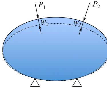
Figure 8.11: An elastic body (structure) loaded by a system of concentrated forces.
