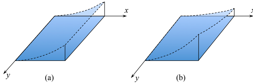
Figure 2.19: (a) cylindrical bending of a plate, and (b) bending with a twist.
