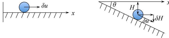
Figure 8.3: Test if an infinitesimal displacement \delta u causes the potential energy to change.
