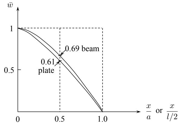
Figure 7.7: Normalized deflected shapes of a beam and a plate is very similar.
