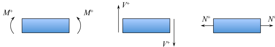
Figure 3.17: Positive shear and normal stresses in a beam.
