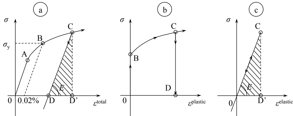
Figure 12.1: Elastic, plastic and total stress-strain curve.
