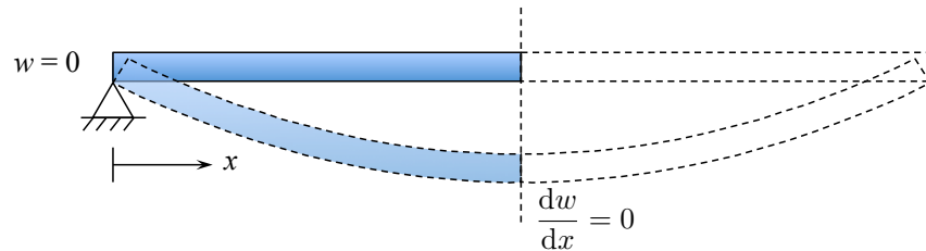
Figure 5.9: Symmetry boundary condition.
