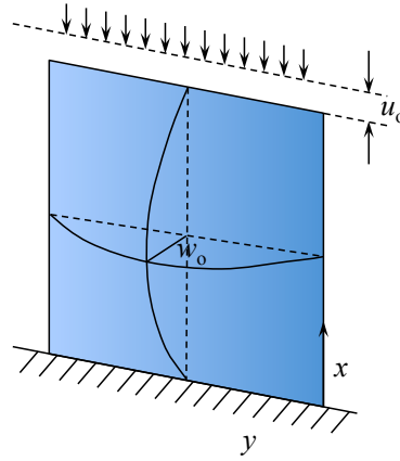
Figure 11.12: Two degree-of-freedom model of the buckled plate.
