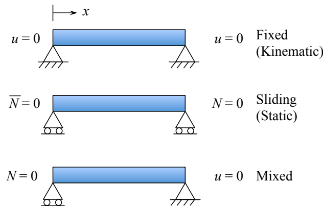
Figure 5.1: Three combinations of in-plane boundary conditions for u(x) .
