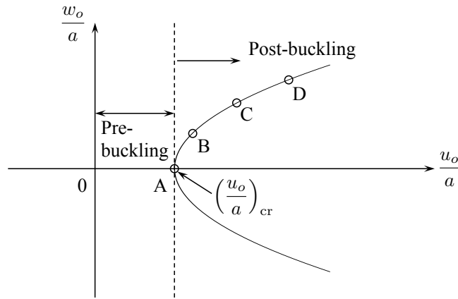
Figure 11.13: The out-of-plane displacement amplitude.
