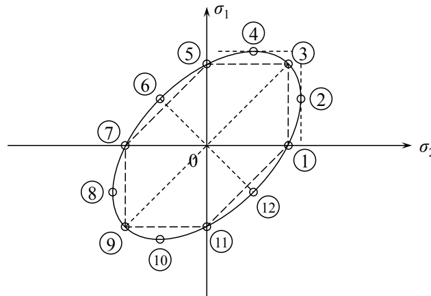
Figure 12.7: The von Mises ellipse in the principal coordinate system.
