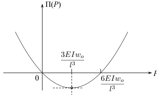
Figure 8.8: Parabolic variation of the total potential energy with the force P for a given central deflection.
