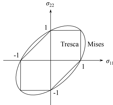
Figure 12.12: Tresca hexagon inscribed into the von Mises ellipse.
