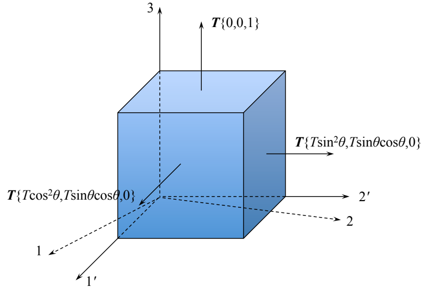
Figure 3.8: Components of the surface tractions on the rotated volume element.
