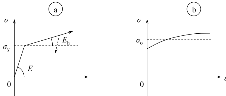
Figure 12.3: Elastic-linear hardening material (a) and rigid-plastic hardening material (b).
