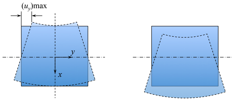
Figure 4.7: Predicted (left) and actual “anticlastic” deformed cross-section of the beam subjected to pure bending. Note that the deflections were magnified by a factor of 10^4 .
