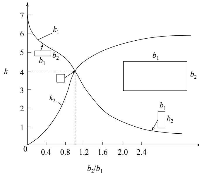
Figure 11.10: Buckling coefficients of a rectangular plate as a function of b_2/b_1 .
