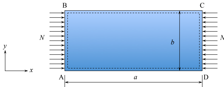
Figure 11.1: Geometry and loading of the classical plate buckling problem.
