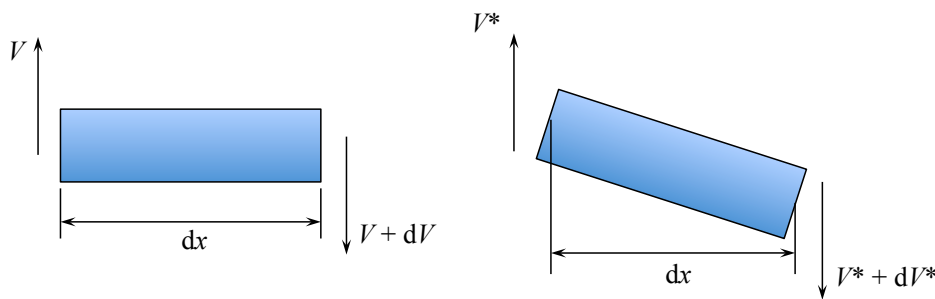
Figure 3.24: Direction of forces to equilibrate the infinitesimal beam element.
