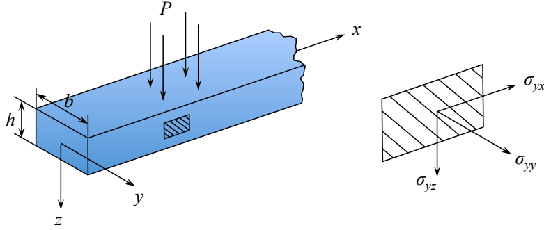
Figure 3.22: Vanishing components of the stress vector.
