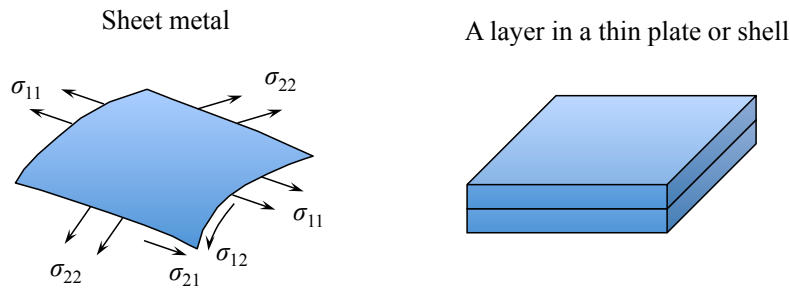
Figure 4.2: Examples of plane stress structures.
