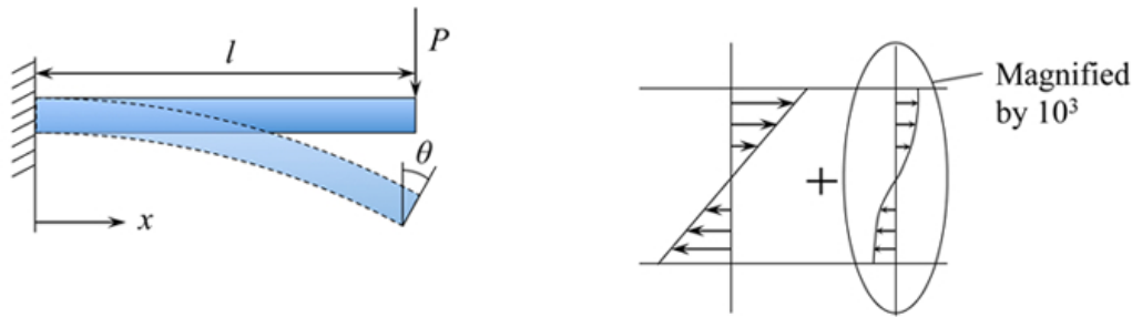
Figure 4.6: Warping of the end section of the cantilever beam.
