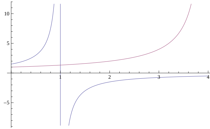
Figure 9.16: The deformation amplitudes B_1 , B_2 vs. load \bar{P} curves, for the case A_1 = 1.5 .
