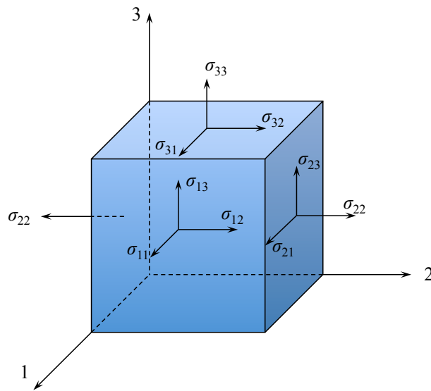
Figure 3.9: Components of the stress tensor on three facets of the infinitesimal surface element.
