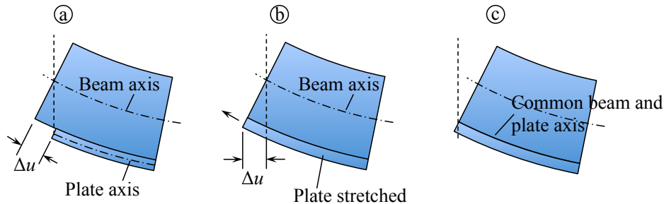
Figure 7.14: Incompatible and compatible interface between beam (stiffener) and plate.
