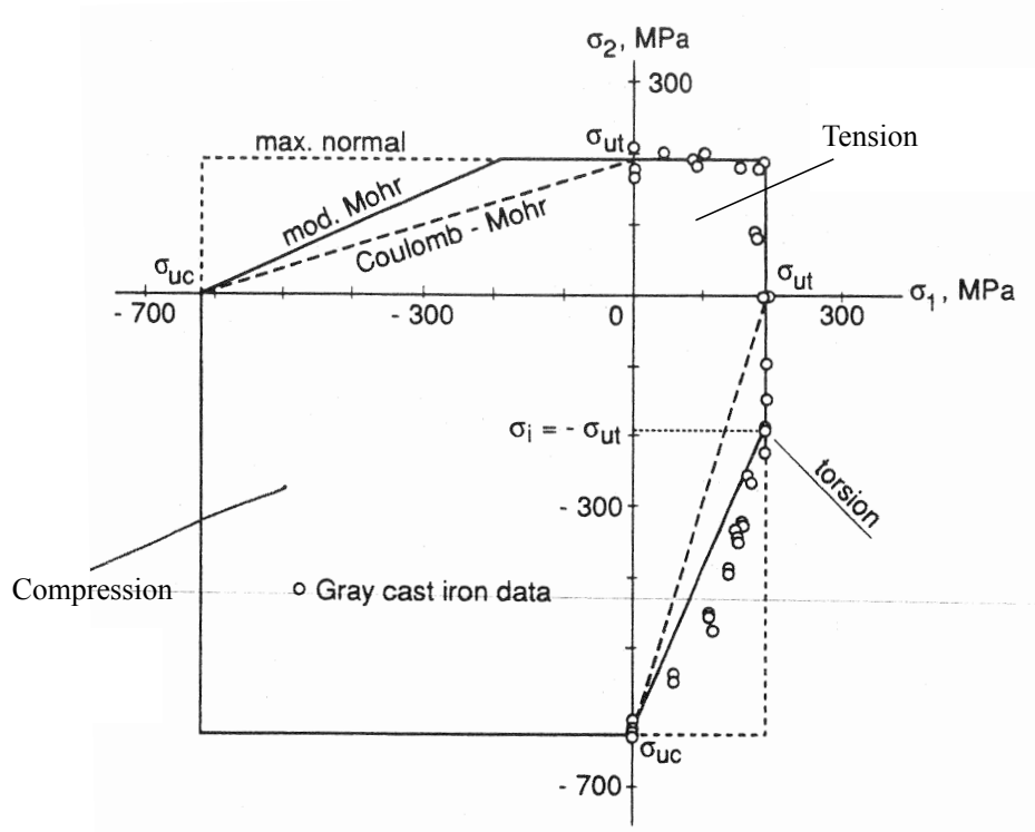
Figure 12.14: Biaxial fracture data of gray cast iron compared to various fracture criteria.
