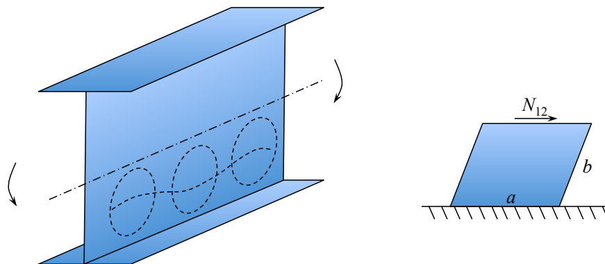
Figure 11.7: Buckling due to shear or bending.
