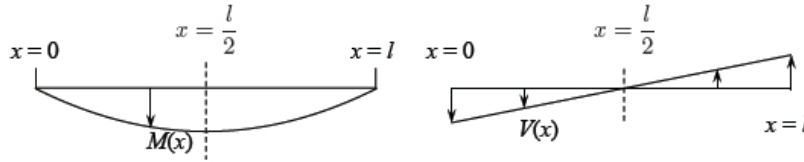
Figure 5.3: Parabolic distribution of the bending moment and linear variation of the shear force.
