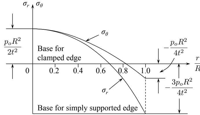
Figure 7.2: Variation of radial and circumferential stresses along the radius of the plate.
