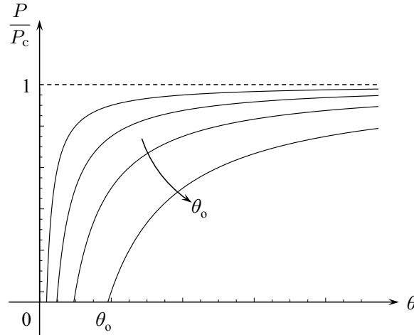
Figure 9.8: A family of equilibrium paths for different values of imperfections.
