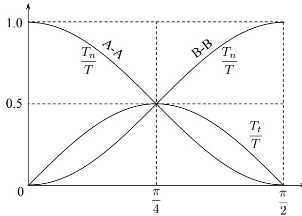
Figure 3.5: Relative values of normal and shear components of the surface traction as a function of the orientation of the cut.
