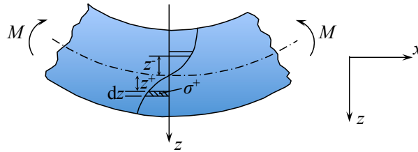
Figure 3.16: The bending moment in a “smiling” beam is positive.
