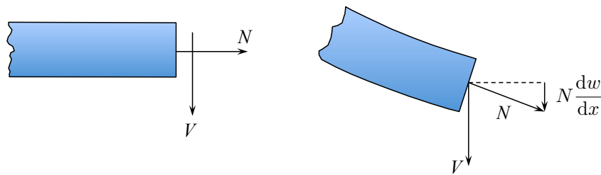
Figure 3.23: In finite rotation the axial force contributes to the total shear force.
