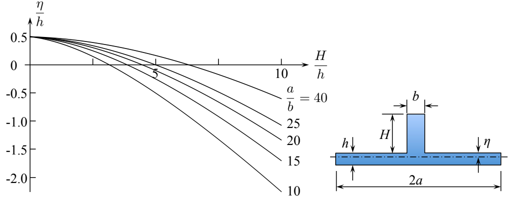
Figure 7.12: Neutral axis of the plate/beam combination moves from the plate center towards the original axis of the beam.
