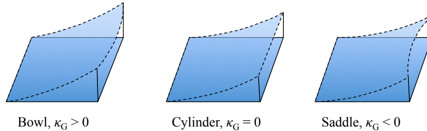
Figure 2.20: Deformed plate with three different classes of shapes.
