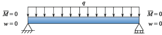
Figure 5.2: Pin support allows for rotation but not for vertical translation.
