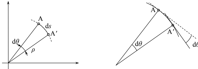
Figure 2.18: Change of slope of a line between two points
