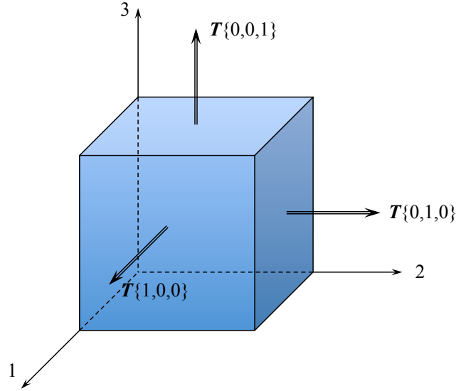
Figure 3.7: The unit volume element aligned with the axis of the bar.
