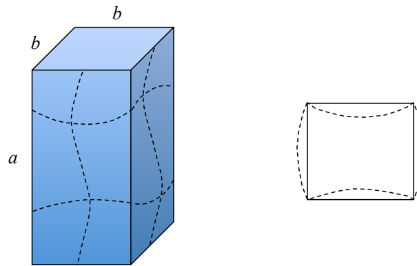
Figure 11.6: The buckling mode of a prismatic square column.
