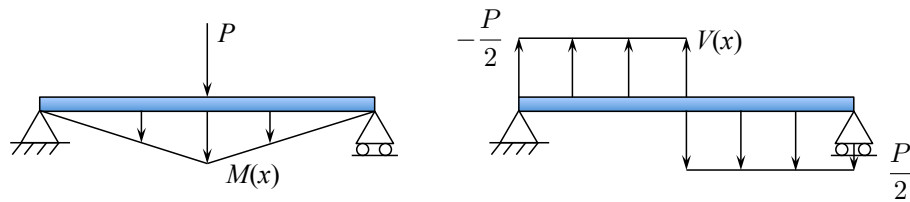
Figure 5.7: Bending moment is continuous at the mid-span, but the shear force is not.
