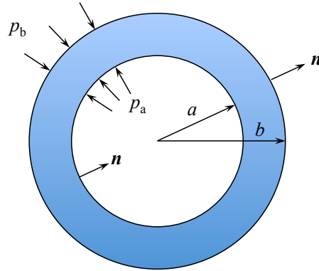
Figure 12.15: Expansion of a thick cylinder by an internal pressure.
