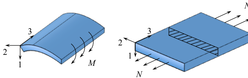
Figure 4.3: Tension of bending of a wide sheet/plate gives rise to plane strain.
