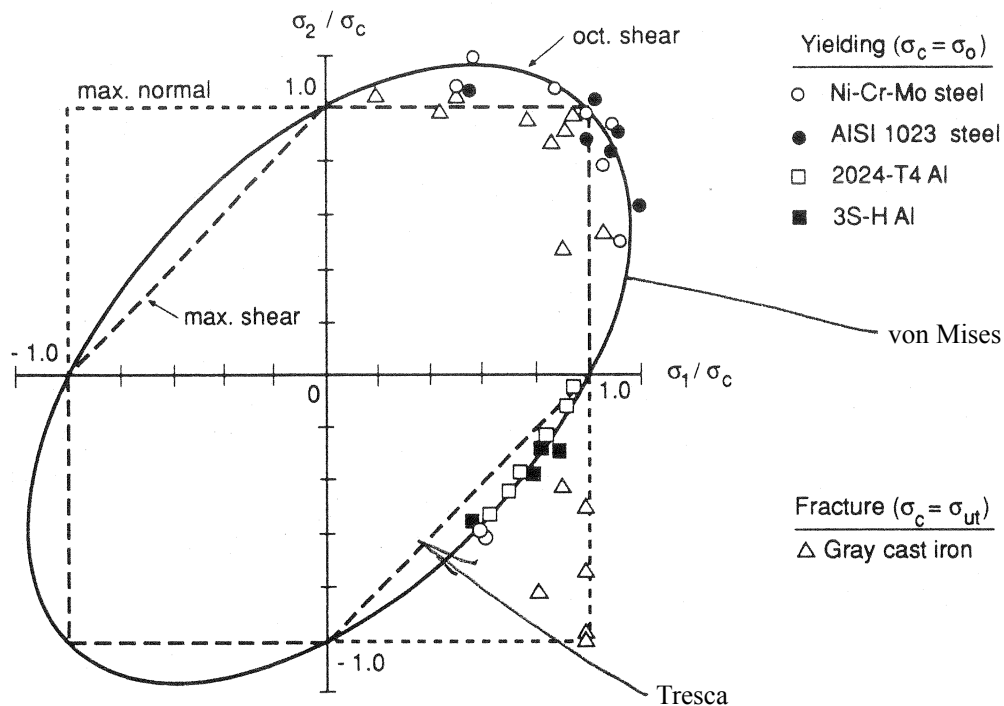
Figure 12.13: Plane stress failure loci for three criteria. These are compared with biaxial yield data for ductile steels and aluminum alloys, and also with biaxial fracture data for gray cast iron.
