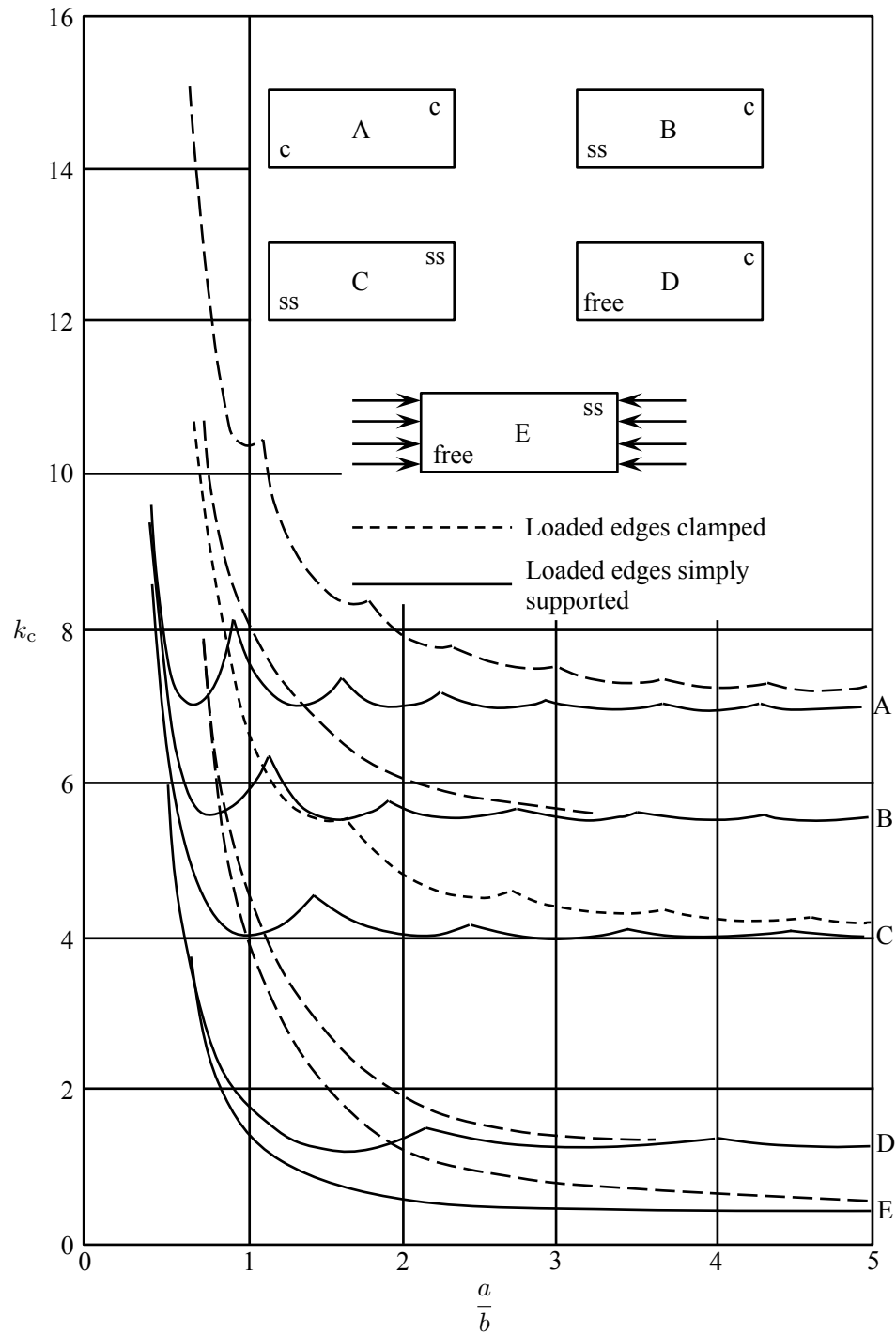
Figure 11.4: Effect of boundary conditions on the buckling coefficient of rectangular plates subjected to in-plane boundary conditions.
