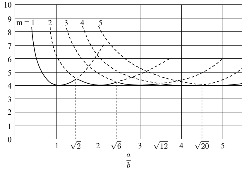
Figure 11.2: Plot of the buckling coefficient for a simply supported plate as a function of the plate aspect ratio a/b and different wave numbers.
