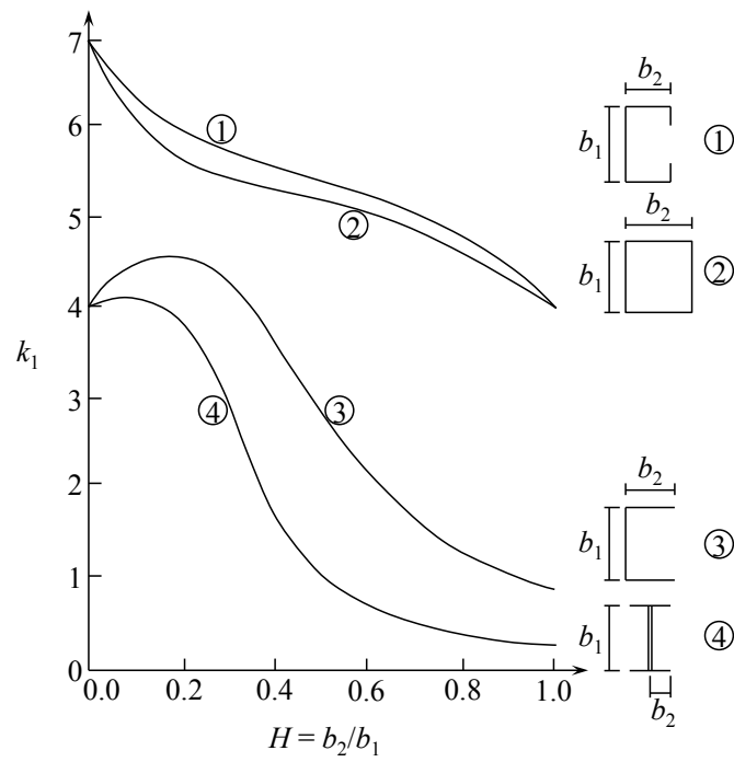
Figure 11.11: Buckling coefficients for four types of sections.
