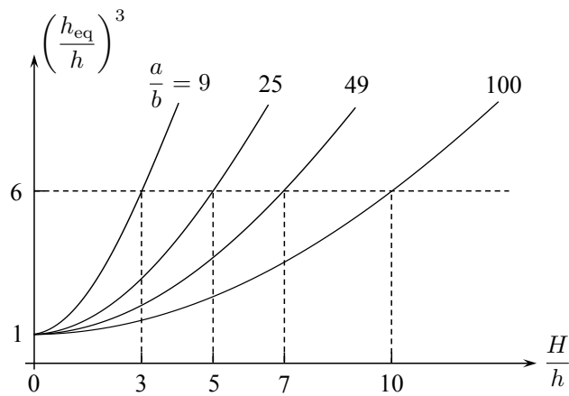
Figure 7.13: The equivalent thickness growth rapidly with the height of the stiffener.
