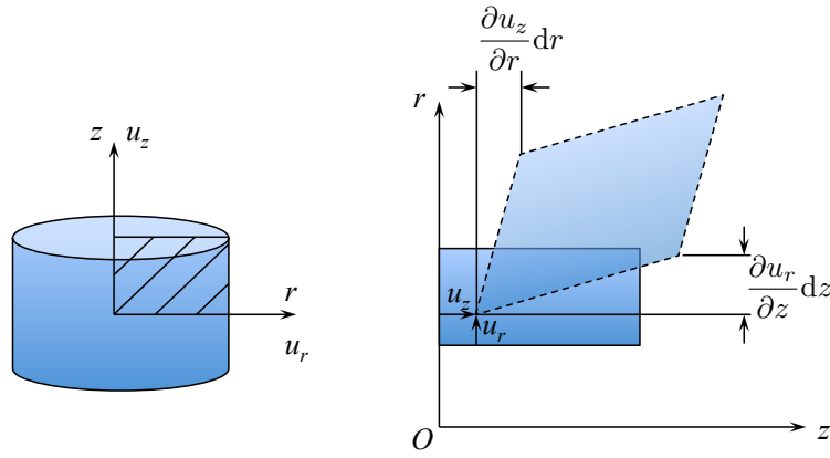
Figure 2.11: Change of angles in the \{r, z\} plane.
