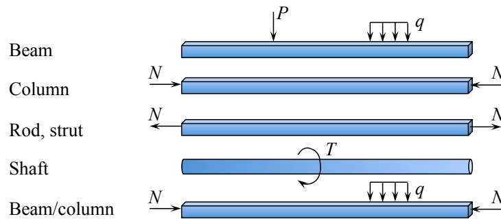
Figure 2.13: The type of loading distinguishes between five different types of structures.
