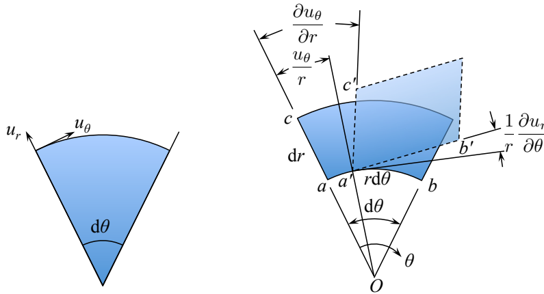
Figure 2.10: Construction that explains change of angles due to radial and circumferential displacement.
