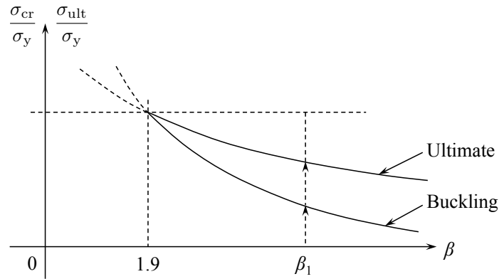
Figure 11.16: Dependence of the buckling stress and ultimate stress on the slenderness ratio.
