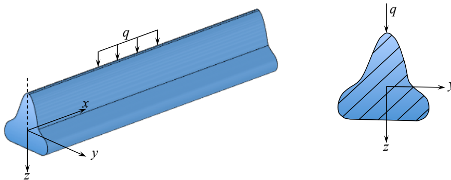
Figure 2.14: A prismatic slender beam with a symmetric cross-section.
