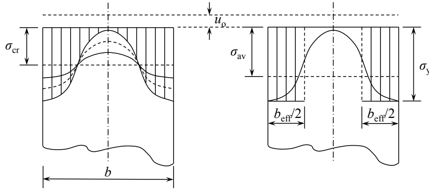
Figure 11.15: Re-distribution of compressive stresses along the loaded edge and simple approximation by von Karman.
