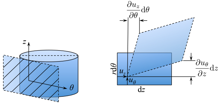
Figure 2.12: Visualization of the strain component \epsilon_{\theta z} .
