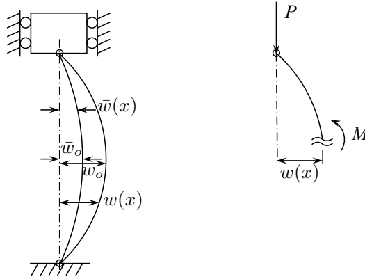
Figure 9.9: A continuous imperfect column and the free body diagram.
