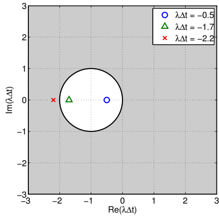
(a) \lambda\Delta t for \lambda = -1
