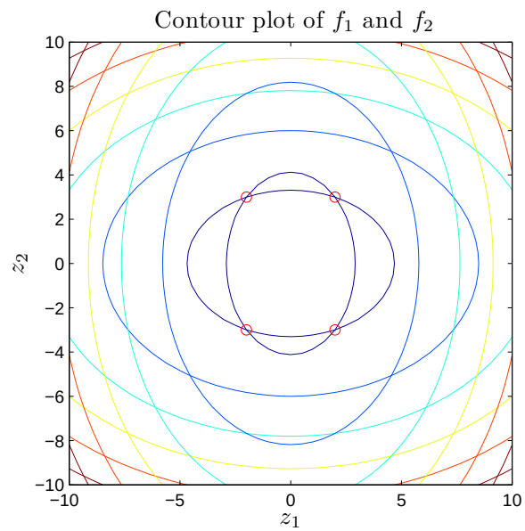
Figure 29.6: Contour plots of f_1 and f_2 with their intersections of the zero contours (the solutions to \mathbf{f}(\mathbf{z}) = \mathbf{0} ) shown as red circles.
