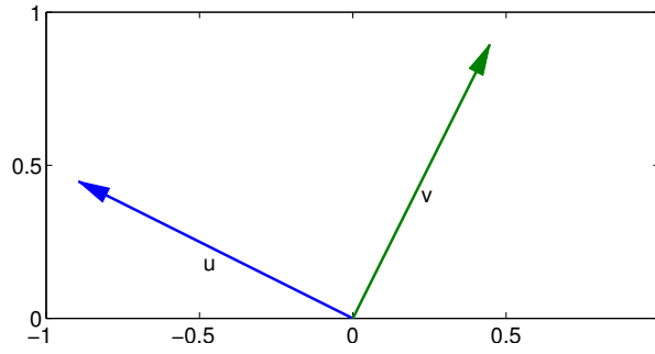
Figure 16.4: An orthonormal set of vectors.
