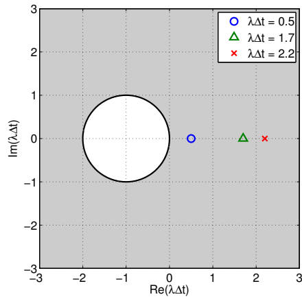
(c) \lambda\Delta t for \lambda = 1
