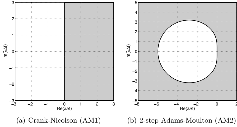
Figure 21.12: The stability diagrams for 2-step Adams-Moulton methods.
