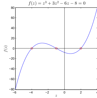
(b) nonlinear function
