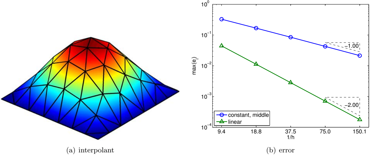
Figure 2.18: Piecewise-linear interpolation
