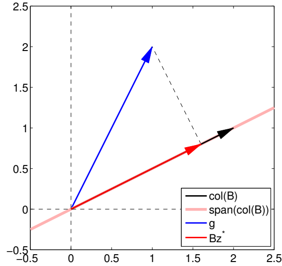
Figure 17.5: Illustration of least-squares in \mathbb{R}^2 .
