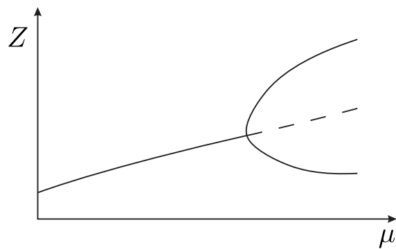
(e) pitchfork
