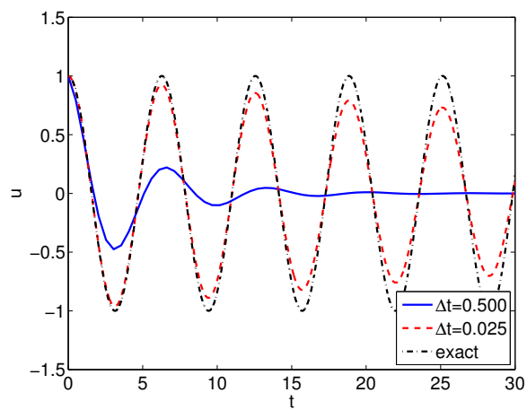
(b) Euler Backward
