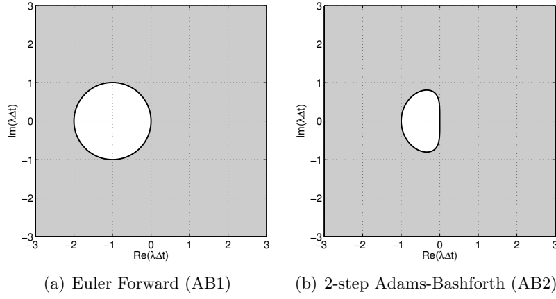
Figure 21.11: The stability diagrams for Adams-Bashforth methods.
