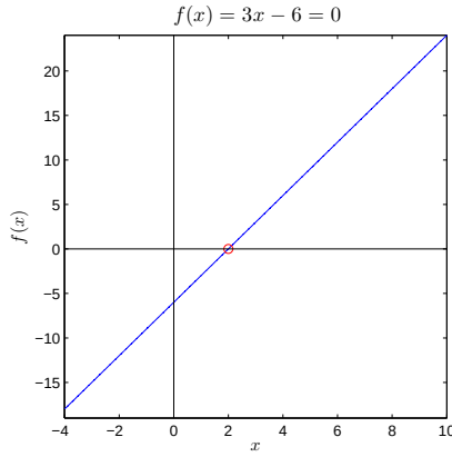
(a) linear function
