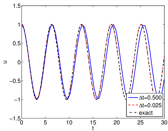
(c) Crank-Nicolson
