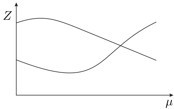
(b) singular point
