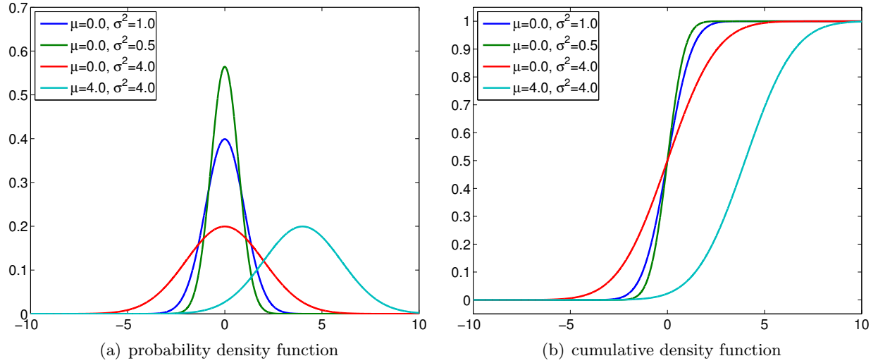
Figure 9.12: Normal distributions
