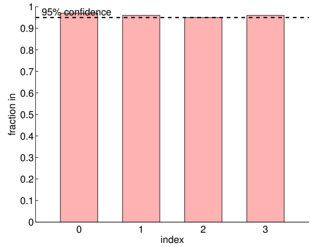
Figure 19.10: Least squares fitting of a quadratic function ( c = 1 ) using a cubic model.
