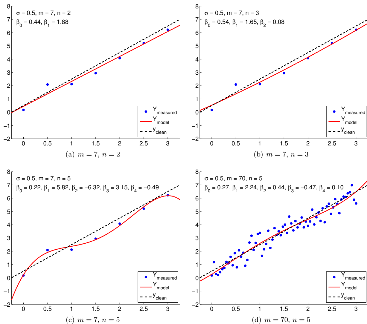
Figure 19.8: Least squares fitting of a linear function using polynomial models of various orders.
