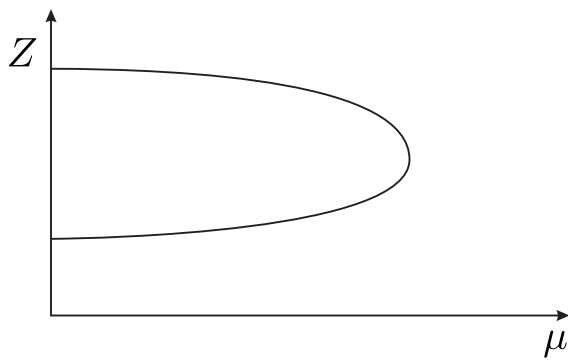
(c) limit point
