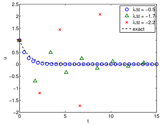
(b) solution ( \lambda = -1 )
