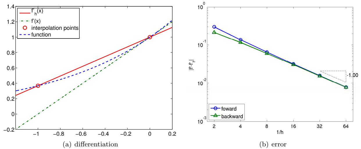
Figure 3.3: Backward difference.
