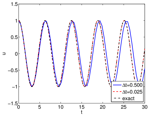
(c) Crank-Nicolson
