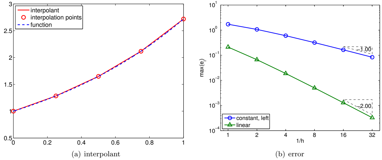
Figure 2.10: Piecewise-linear interpolant.
