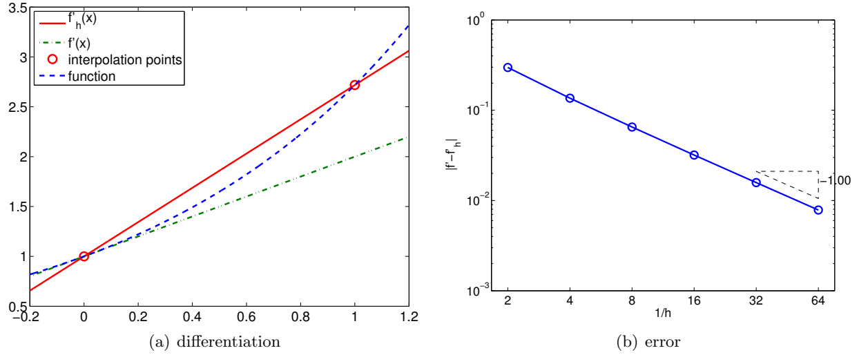
Figure 3.2: Forward difference.
