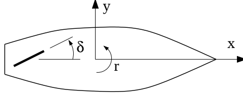
Figure 3: Convention for positive rudder angle in the vessel reference system.
