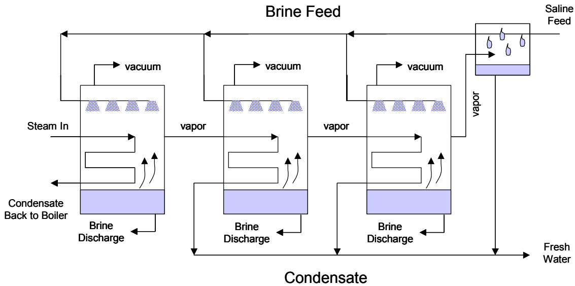
Figure 6. Schematic of multi-effect evaporator desalination process (horizontal tube – parallel feed configuration).
