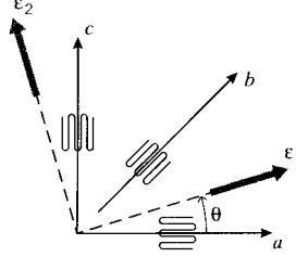
Figure 4: Strain rosette.
