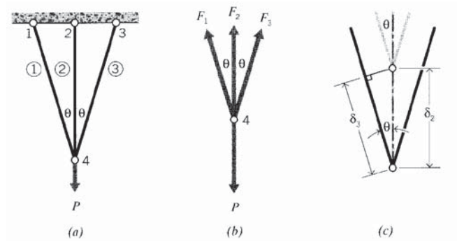
Figure 11: (a) Three-element statically indeterminate truss. (b) Free-body diagram of node 4. (c) Deflections at node 4.
