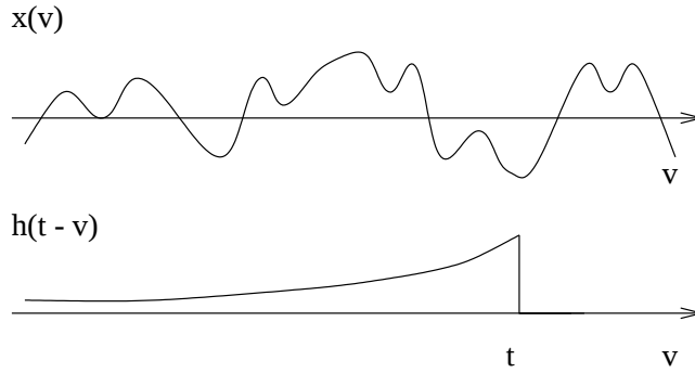
FIGURE 9.6 Illustration of the two terms in the integrand of Eqn. (9.56)
