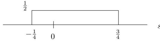
FIGURE 8.4 Plot of f_{R|S}(\frac{1}{4}|s)f_S(s) .
