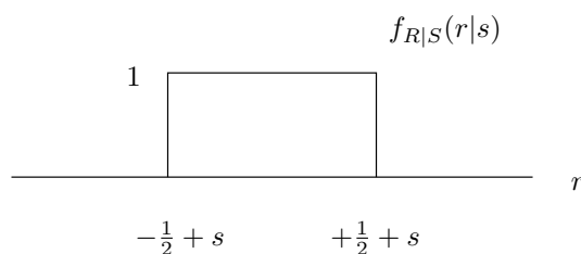
FIGURE 8.2 Conditional PDF of R given S , f_{R|S}(r|s) .
