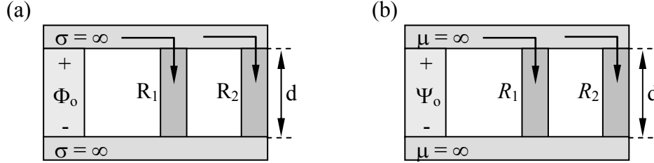
Figure 4.4.1 Current and magnetic flux-divider circuits.
