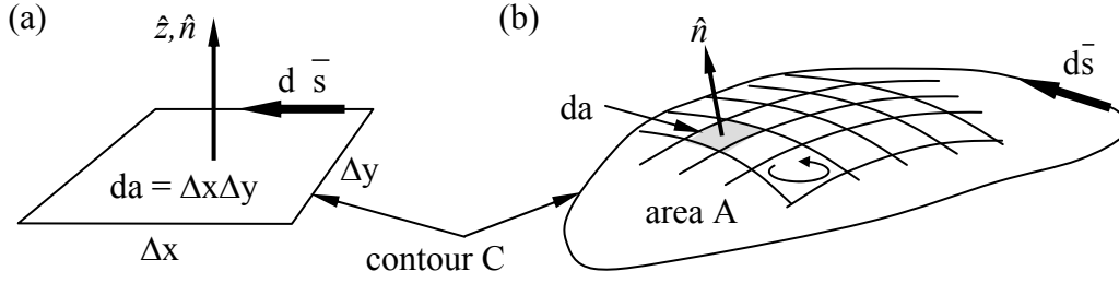
Figure 2.4.2 Derivation of Stokes' theorem.
