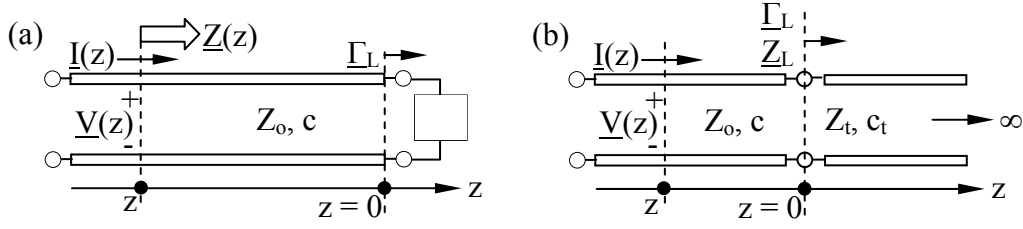
Figure 7.2.2 TEM transmission line impedances and coupling.
