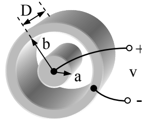
Figure 3.1.4 Cylindrical capacitor.
