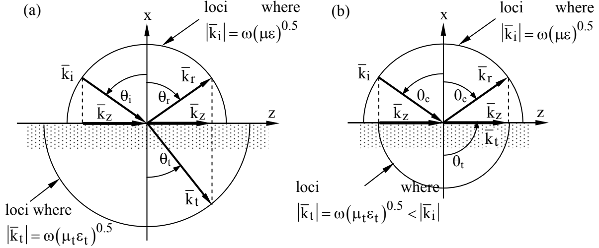
Figure 9.2.3 Angles of reflection and transmission, and the critical angle \theta_c .
