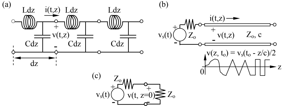
Figure 8.1.1 Distributed circuit model for lossless TEM transmission lines.
