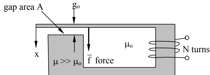
Figure 6.3.7 Magnetic relay.
