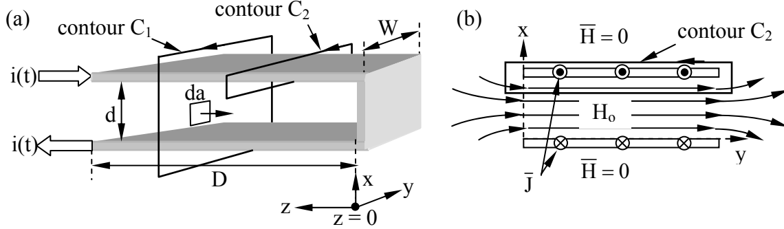
Figure 3.2.1 Parallel-plate inductor.
