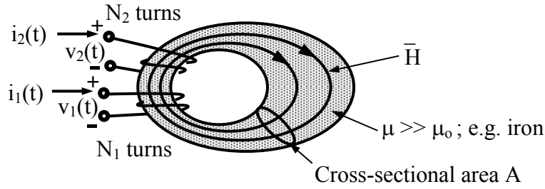
Figure 3.2.7 Toroidal transformer.
