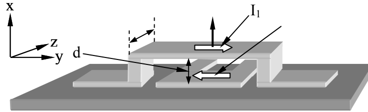
Figure 6.4.2 Magnetic MEMS switch.
