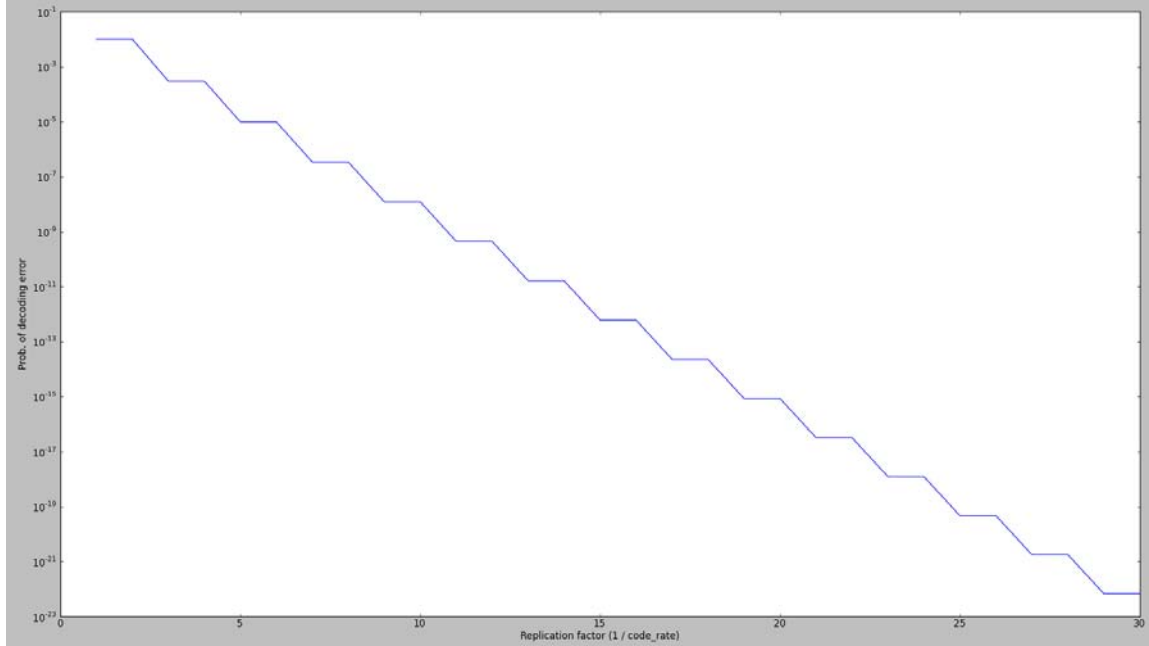
Figure 5-1: Probability of a decoding error with the repetition code that replaces each bit b with n copies of b . The code rate is 1/n .
