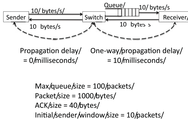
Figure 19-9: Ben's network.
