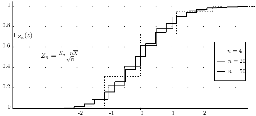
Figure 1.11: The same CDF's as Figure 1.5 normalized to 0 mean and unit standard deviation, i.e., the CDF's of Z_n = (S_n/n - \bar{X}) \frac{\sqrt{n}}{\sigma} for n = 4, 20, 50 . Note that as n increases, the CDF of Z_n slowly starts to resemble the normal CDF.
