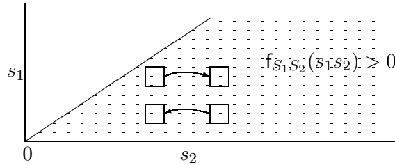
Figure 2.4: The joint density of S_1, S_2 is non-zero in the region shown. It can be changed, while holding the marginals constant, by reducing the joint density by \epsilon in the upper left and lower right squares above and increasing it by \epsilon in the upper right and lower left squares.
