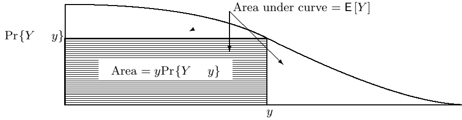
Figure 1.7: Demonstration that y\Pr\{Y > y\} \leq \mathbf{E}[Y] . By letting y \rightarrow \infty , it can also be seen that the shaded area becomes a negligible portion of the area \mathbf{E}[Y] , so that \lim_{y \rightarrow \infty} y\Pr\{Y > y\} = 0 if \mathbf{E}[Y] < \infty .
