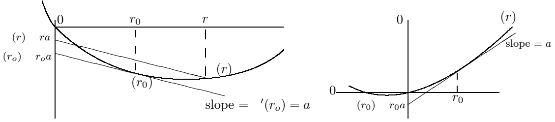
Figure 1.9: Graphical minimization of (r) - ar : For any r \in I(X) , (r) - ar is the vertical axis intercept of a line of slope a through the point (r, (r)) . The minimum occurs when the line of slope a is tangent to the curve. The two examples show one case where E[X] < 0 and another where E[X] > 0 .
