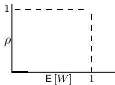
Figure 5.8: \rho as a function of E[W] for given d .
