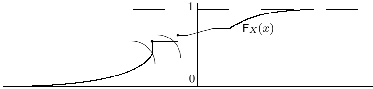
Figure 1.1: Example of a CDF for a rv that is neither continuous nor discrete. If F_X(x) has a discontinuity at some x_o , it means that there is a discrete probability at x_o equal to the magnitude of the discontinuity. In this case F_X(x_o) is given by the height of the upper point at the discontinuity.
