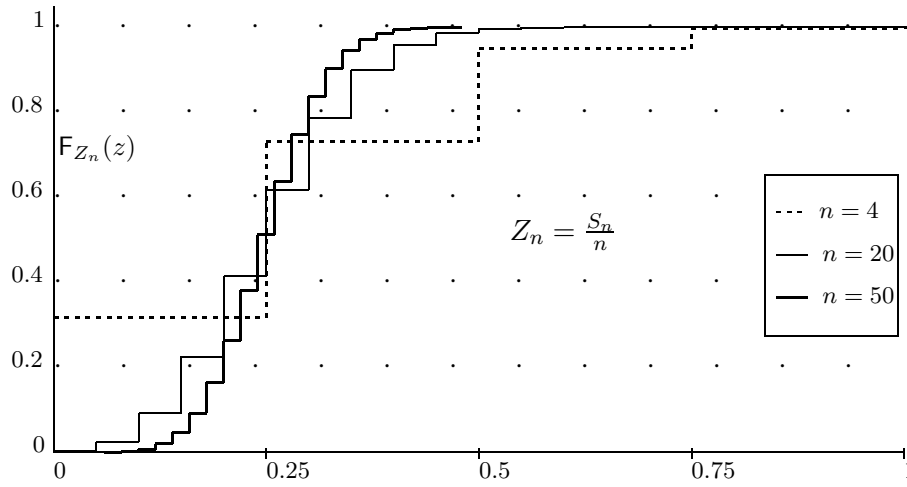
Figure 1.9: The same CDF as Figure 1.5, scaled differently to give the CDF of the sample average Z_n . It can be visualized that as n increases, the CDF of Z_n becomes increasingly close to a unit step at the mean, 0.25, of the variables X being summed.
