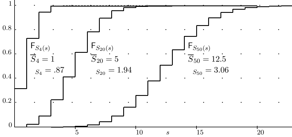
Figure 1.5: The CDF F_{S_n}(s) of S_n = X_1 + \dots + X_n where X_1, \dots, X_n are typical IID rv's and n takes the values 4, 20, and 50. The particular rv X in the figure is binary with p_X(1) = 1/4 , p_X(0) = 3/4 . Note that the mean of S_n is proportional to n and the standard deviation to \sqrt{n} .
