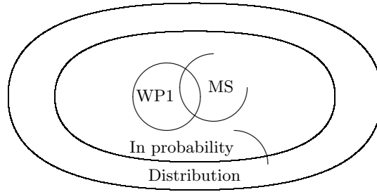
Figure 1.14: Relationship between different kinds of convergence: Convergence in distribution is the most general and is implied by all the others. Convergence in probability is the next most general and is implied both by convergence with probability 1 (WP1) and by mean square (MS) convergence, neither of which implies the other.
