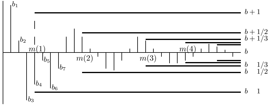
Figure 1.15: Illustration of a sequence of real numbers b_1, b_2, \dots that converge to a number b . The figure illustrates an integer m(1) such that for all n \geq m(1) , b_n lies in the interval b \pm 1 . Similarly, for each k \geq 1 , there is an integer m(k) such that b_n lies in b \pm 1/k for all n \geq m(k) . Thus \lim_{n \rightarrow \infty} b_n = b means that for a sequence of ever tighter constraints, the k th constraint can be met for all sufficiently large n , (i.e., all n \geq m(k) ). Intuitively, convergence means that the elements b_1, b_2, \dots get close to b and stay close. The sequence of positive integers m(1), m(2), \dots is non-decreasing, but otherwise arbitrary, depending only on the sequence \{b_n; n \geq 1\} . For sequences that converge very slowly, the integers m(1), m(2), \dots are simply correspondingly larger.
