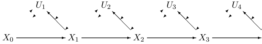
Figure 6.17: The statistical dependencies between the rv's of a semi-Markov process. Each holding interval U_n , conditional on the current state X_{n-1} and next state X_n , is independent of all other states and holding intervals. Note that, conditional on X_n , the holding intervals U_n, U_{n-1}, \dots , are statistically independent of U_{n+1}, X_{n+2}, \dots .
