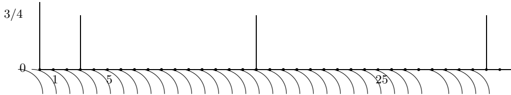
Figure 1.17: Illustration of a sample path of a sequence of rv's \{Y_n; n \geq 0\} where, for each j \geq 0 , Y_n = 1 for an equiprobable choice of n \in [5^j, 5^{j+1}) and Y_n = 0 otherwise.
