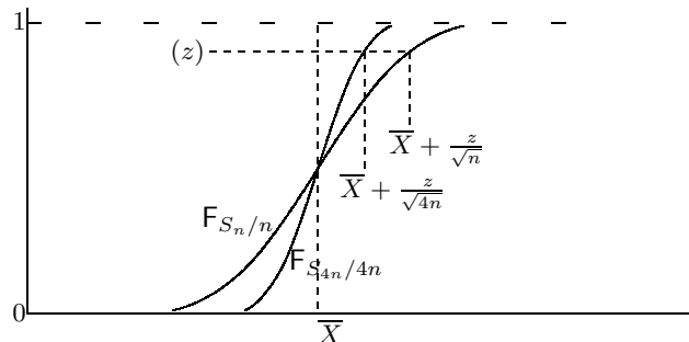
Figure 1.12: Approximation of the CDF F_{S_n/n} of a sample average by a Gaussian distribution of the same mean and variance. The WLLN says that F_{S_n/n} approaches a step function at \bar{X} as n \rightarrow \infty . The CLT says that the shape of S_n/n approximates a Gaussian distribution \mathcal{N}(\bar{X}, \sigma^2/n) . If n is increased by a factor of 4, the Gaussian distribution curve is horizontally scaled inward toward \bar{X} by a factor of 2. The CLT says both that the CDF of S_n/n is scaled horizontally as 1/\sqrt{n} and also that it is better approximated by the Gaussian of the given mean and variance as n increases.
