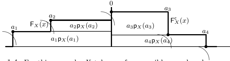
Figure 1.4: For this example, X takes on four possible sample values, a_1 < a_2 < 0 < a_3 < a_4 . The figure plots F_X(x) for x \leq 0 and F_X^c(x) for x > 0 . As in Figure 1.3, \int_{x=0}^{\infty} F_X^c(x) dx = a_3 f_X(a_3) + a_4 f_X(a_4) . Similarly, \int_{x=-\infty}^0 F_X(x) dx = a_1 f_X(a_1) + a_2 f_X(a_2) .
