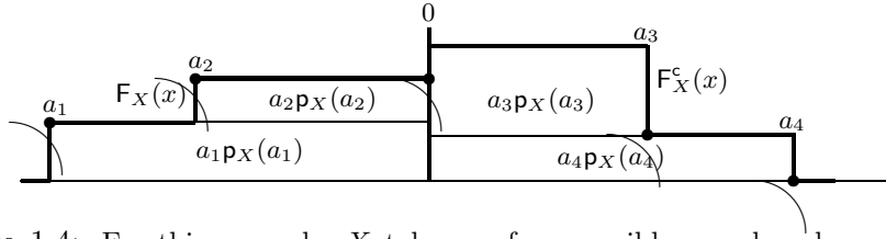
Figure 1.4: For this example, X takes on four possible sample values, a_1 < a_2 < 0 < a_3 < a_4 . The figure plots F_X(x) for x \leq 0 and F_X^c(x) for x > 0 . As in Figure 1.3, \int_0^\infty F_X^c(x) dx = a_3 p_X(a_3) + a_4 p_X(a_4) . Similarly, \int_{-\infty}^0 F_X(x) dx = a_1 p_X(a_1) + a_2 p_X(a_2) .
