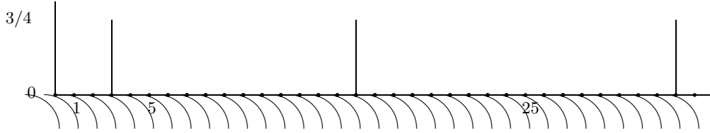
Figure 1.18: Illustration of a sample path of a sequence of rv's \{Y_n; n \geq 0\} where, for each j \geq 0 , Y_n = 1 for an equiprobable choice of n \in [5^j, 5^{j+1}) and Y_n = 0 otherwise.
