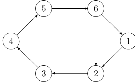
Figure 3.4: An ergodic chain with M = 6 states in which P_{ij}^m > 0 for all m > (M - 1)^2 and all i, j but P_{11}^{(M-1)^2} = 0 . The figure also illustrates that an M state Markov chain must have a cycle with M - 1 or fewer nodes. To see this, note that an ergodic chain must have cycles, since each node must have a walk to itself, and subcycles of repeated nodes can be omitted from that walk, converting it into a cycle. Such a cycle might have M nodes, but a chain with only an M node cycle would be periodic. Thus some nodes must be on smaller cycles, such as the cycle of length 5 in the figure.
