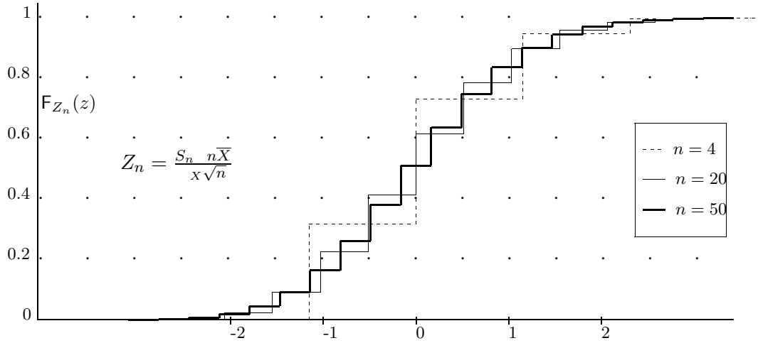
Figure 1.12: The same distribution functions as Figure 1.5 normalized to 0 mean and unit standard deviation, i.e., the distribution functions of Z_n = (S_n/n - \bar{X}) \frac{\sqrt{n}}{s} for n = 4, 20, 50 . Note that as n increases, the distribution function of Z_n slowly starts to resemble the normal distribution function.
