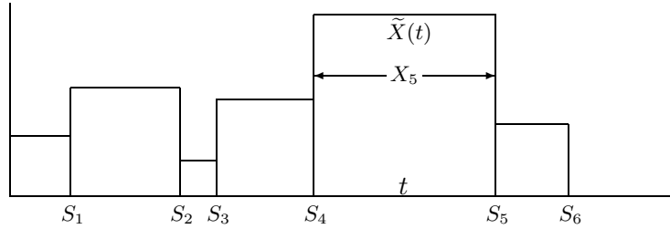
Figure 4.8: Duration \tilde{X}(t) = X_{N(t)+1} of the inter-renewal interval containing t .
