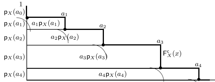
Figure 1.3: The figure shows the complementary CDF F_X^c of a nonnegative discrete rv X . For this example, X takes on five possible values, 0 = a_0 < a_1 < a_2 < a_3 < a_4 . Thus F_X^c(x) = \Pr\{X > x\} = 1 - p_X(a_0) for x < a_1 . For a_1 \leq x < a_2 , \Pr\{X > x\} = 1 - p_X(a_0) - p_X(a_1) , and \Pr\{X > x\} has similar drops as x reaches a_2 , a_3 , and a_4 . E[X] , from (1.28), is \sum_i a_i p_X(a_i) , which is the sum of the rectangles in the figure. This is also the area under the curve F_X^c(x) , i.e., \int_0^\infty F_X^c(x) dx . It can be seen that this argument applies to any nonnegative rv, thus verifying (1.30).
