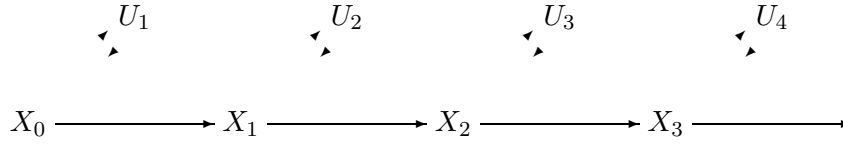
Figure 6.1: The statistical dependencies between the rv's of a Markov process. Each holding interval U_i , conditional on the current state X_{i-1} , is independent of all other states and holding intervals.
