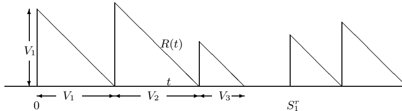
Figure 4.16: Sample value of the residual life function of customers in service.
