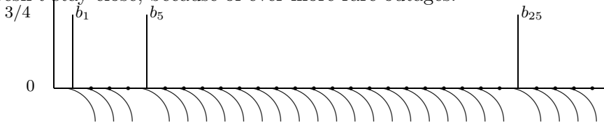
Figure 1.16: Illustration of a non-convergent sequence of real numbers b_1, b_2, \dots . The sequence is defined by b_n = 3/4 for n = 1, 5, 25, \dots, 5^j, \dots for all integer j \geq 0 . For all other n , b_n = 0 . The terms for which b_n \neq 0 become increasingly rare as n \rightarrow \infty . Note that b_n \in [-1, 1] for all n , but there is no m(2) such that b_n \in [-1/2, 1/2] for all n \geq m(2) . Thus the sequence does not converge.
