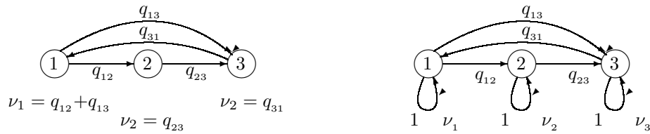
Figure 6.6: Approximating a generic Markov process by its sampled-time Markov chain.
