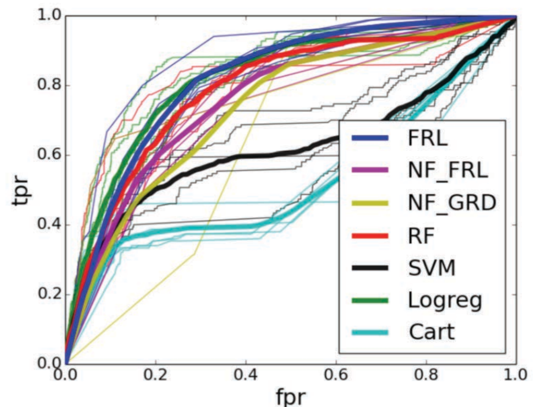
32 Figure 2: ROC curves for readmissions prediction.
