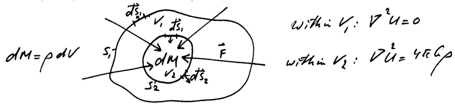
Figure 2.11: Applicability of Poisson's and Laplace's equations.
