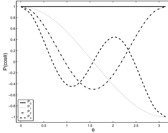
Figure 2.13: Legendre polynomials.
