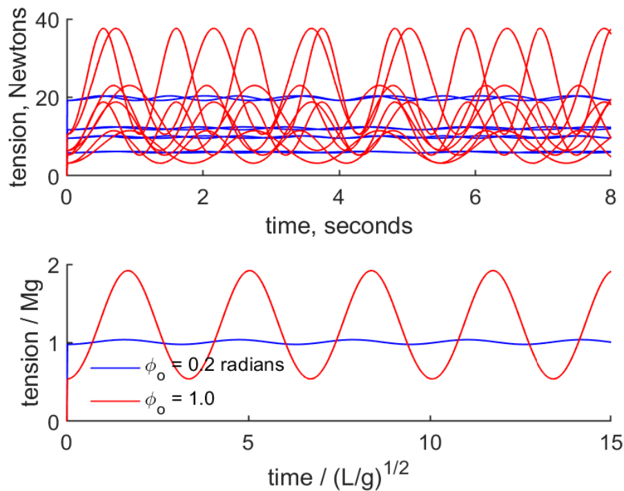
Figure 1: This essay is an introduction to dimensional analysis, one of the most valuable tools of applied mathematics. The essential idea is a change of variables from the usual dimensional variables to nondimensional variables that are formed from scales natural to the phenomenon. An immediate benefit, illustrated here, is that the nondimensional variables will be fewer in number than the dimensional variables. These data are tension in the line of a simple pendulum computed during 16 numerical experiments. In the upper panel, these data are shown in dimensional coordinates, time in seconds and tension in Newtons. In the lower panel, the same data are shown in nondimensional coordinates defined from natural scales of a pendulum: time is scaled by (nondimensionalized by) the reduced period of small amplitude oscillation, \sqrt{L/g} , and tension is scaled by the weight of the bob, Mg . With these choices, the 16 distinct dimensional solutions collapse into two solutions that differ only by their initial angular displacement, \phi_o , large or small amplitude (red or blue lines). These graphs present the same data, but the nondimensional version is far more legible. Better still, it applies to all similar simple pendulums (similar in this case means the same \phi_o ).
