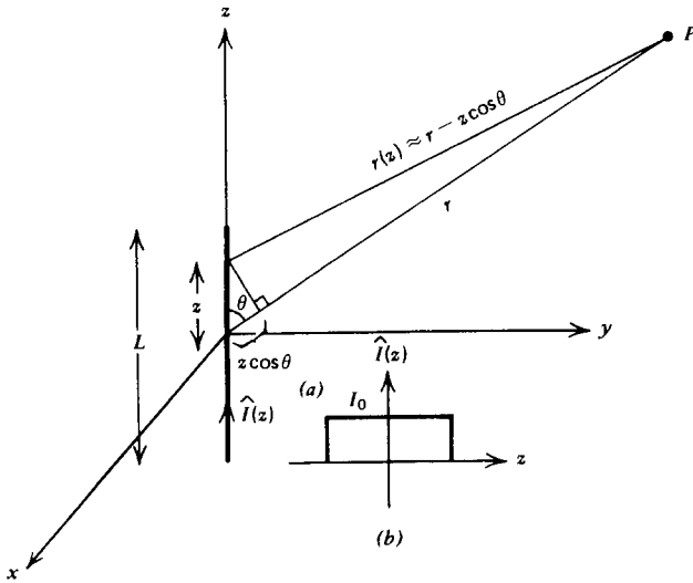
Figure 9-11 (a) For a long dipole antenna, each incremental current element at coordinate z is at a slightly different distance to any field point P . (b) The simplest case study has the current uniformly distributed over the length of the dipole.
