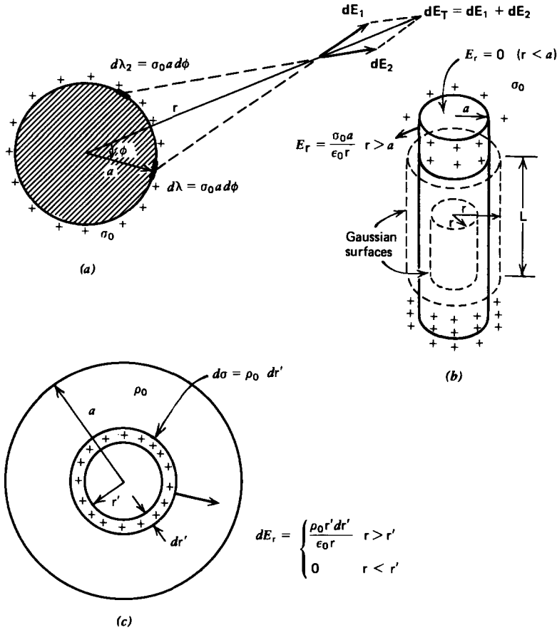
Figure 2-18 (a) Symmetrically located line charge elements on a cylinder with uniformly distributed surface charge show that the electric field is purely radial. (b) Gauss's law applied to concentric cylindrical surfaces shows that the field inside the surface charged cylinder is zero while outside it is the same as if all the charge per unit length \sigma_0 2\pi a were concentrated at the origin as a line charge. (c) In addition to using the surfaces of (b) with Gauss's law for a cylinder of volume charge, we can also sum the contributions from incremental hollow cylinders of surface charge.
