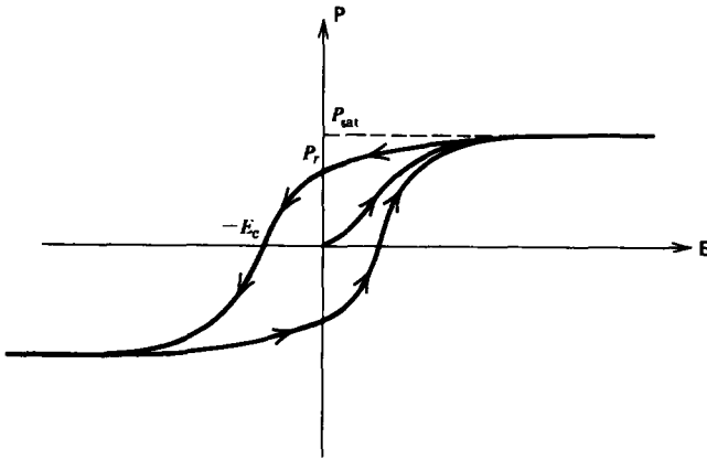
Figure 3-8 A typical ferro-electric hysteresis curve shows a saturation value P_{sat} , when all the domains align with the field, a remanent polarization P_r , when the electric field is removed, and a negative coercive electric field -E_c , necessary to bring the polarization back to zero.
