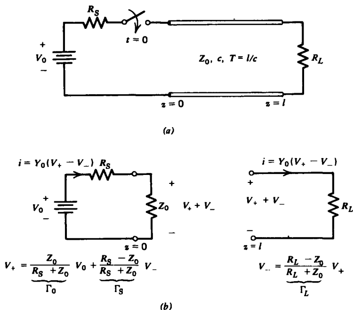
Figure 8-8 (a) A dc voltage V_0 is switched onto a resistively loaded transmission line through a source resistance R_s . (b) The equivalent circuits at z = 0 and z = l allow us to calculate the reflected voltage wave amplitudes in terms of the incident waves.
