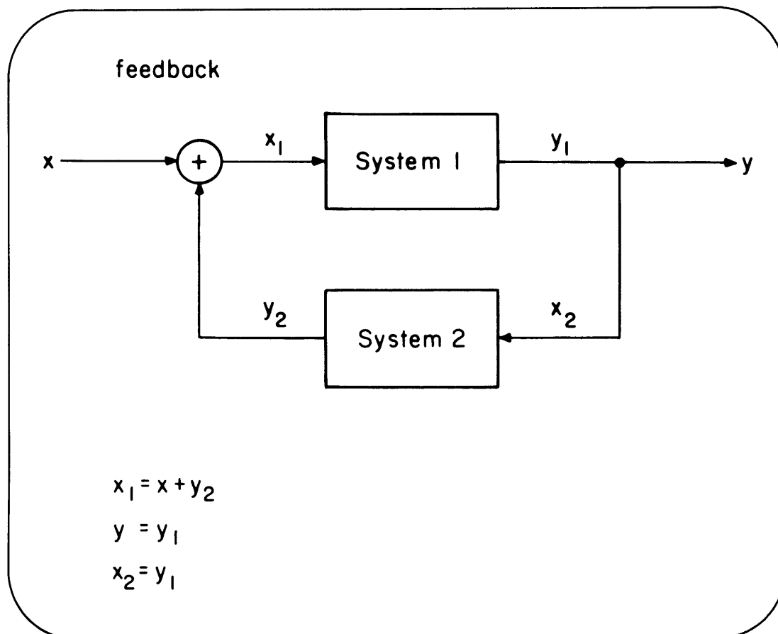
TRANSPARENCY 3.12 Feedback inter-connection of two systems.
