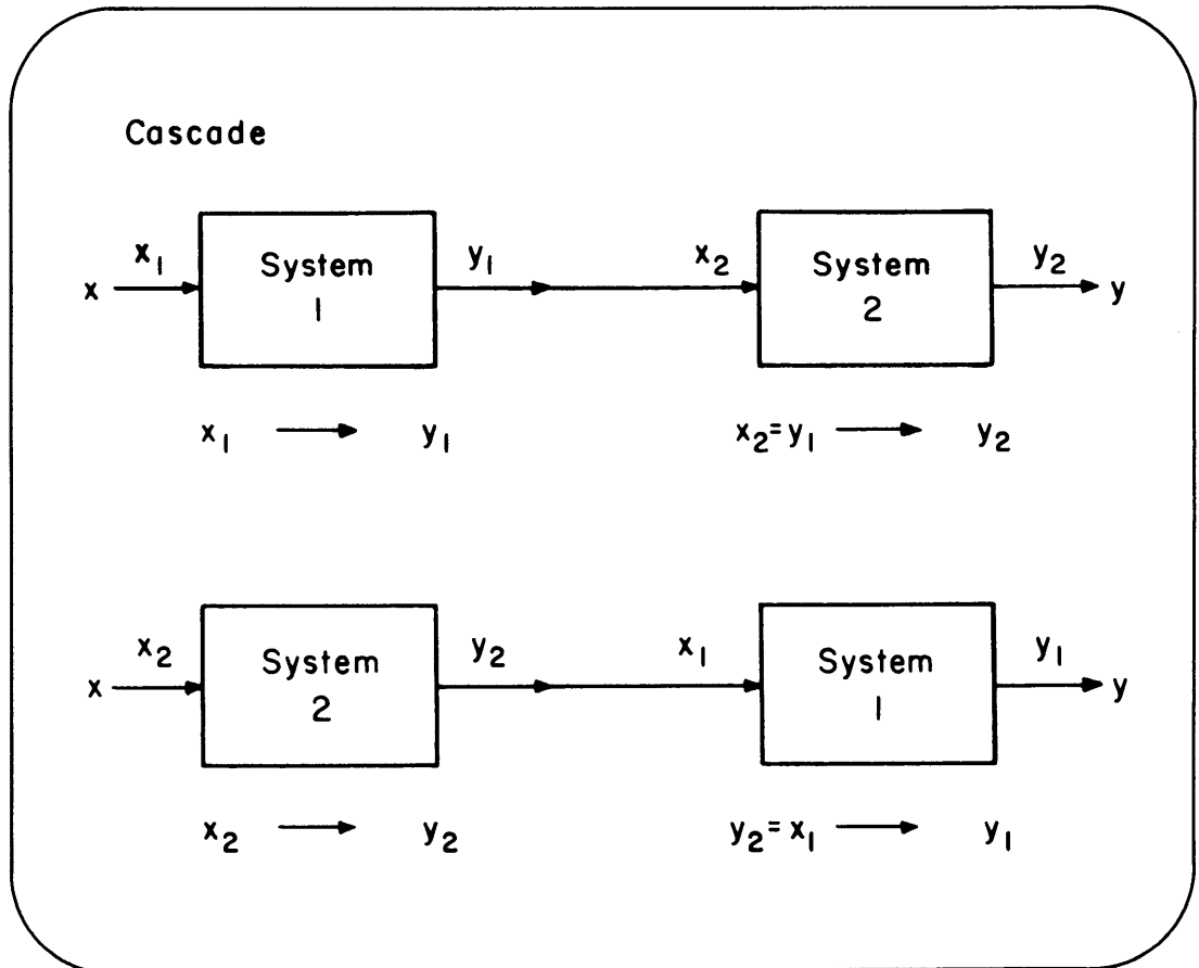
TRANSPARENCY 3.10 Interconnection of two systems in cascade.
