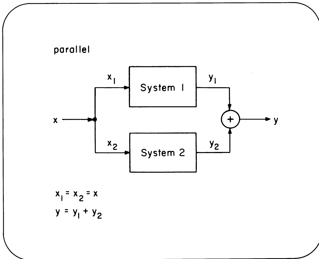
TRANSPARENCY 3.11 Interconnection of two systems in parallel.
