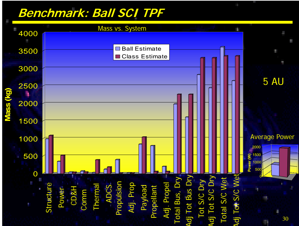
Benchmark: Ball SCI TPF 5AU Mass in kg, Power in watts
