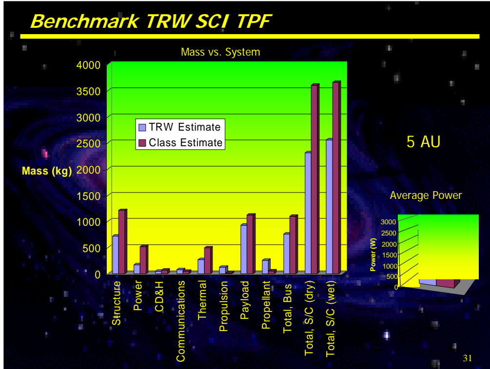
Benchmark: TRW SCI TPF 5AU
